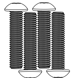
allen bolt M8*35L ( 4 ) PCS
