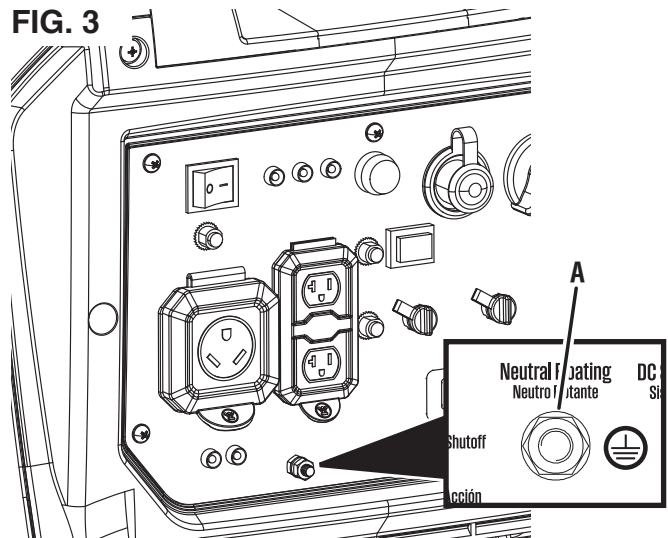
A - Ground terminal
