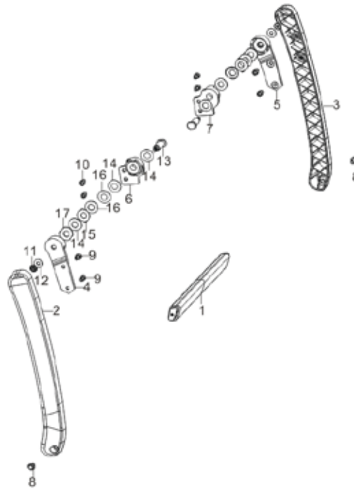
FIG. 15. WHEEL ASSEMBLY
