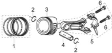
FIG. 5. PISTON RING SET & CONNECTING ROD
