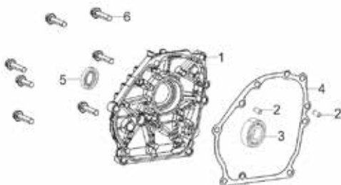
FIG. 2. CRANKCASE COVER ASSEMBLY
