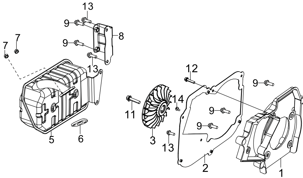
Fig. 11 - Muffler Assembly
