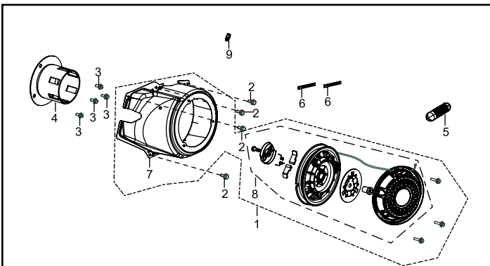
Fig. 7 - Recoil Starter
