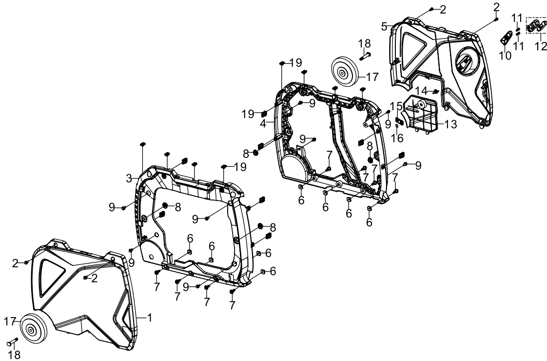
Fig. 16 - Side Covers
