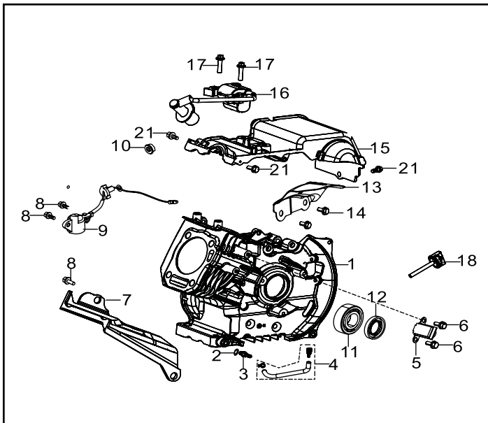
Fig. 1 - Crankcase Assembly
