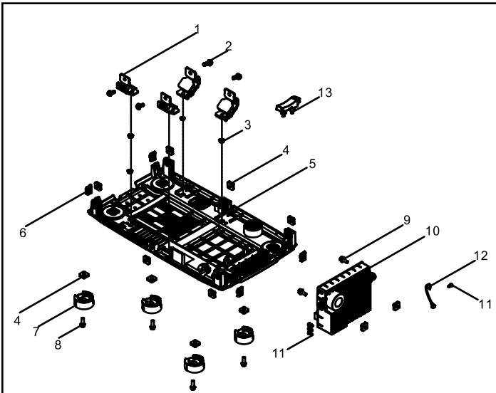
Fig. 12 - Bottom Plate, Inverter
