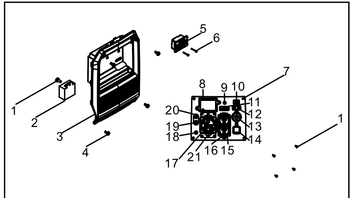
Fig. 10 - Control Panel
