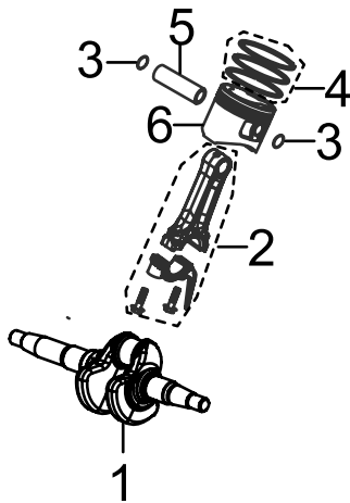
Fig. 3 - Crankshaft & Piston
