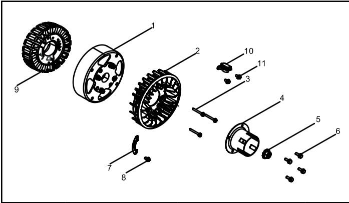
Fig. 7 - Flywheel & Alternator
