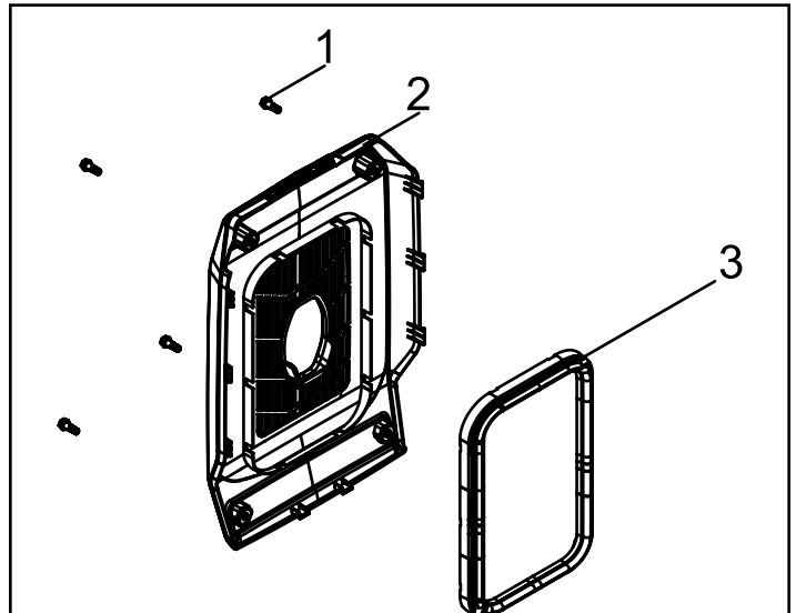
Fig. 13 - Muffler Cover
