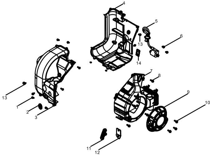
Fig. 5 - Recoil Starter
