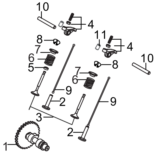
Fig. 4 - Valve Train, Camshaft
