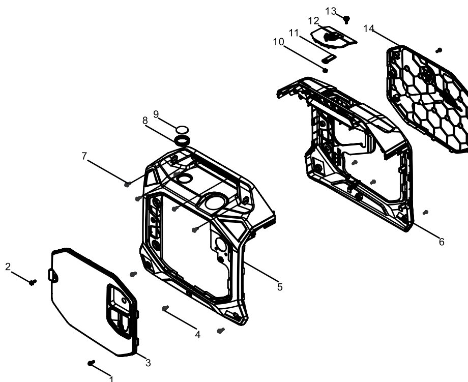
Fig. 11 - Housing
