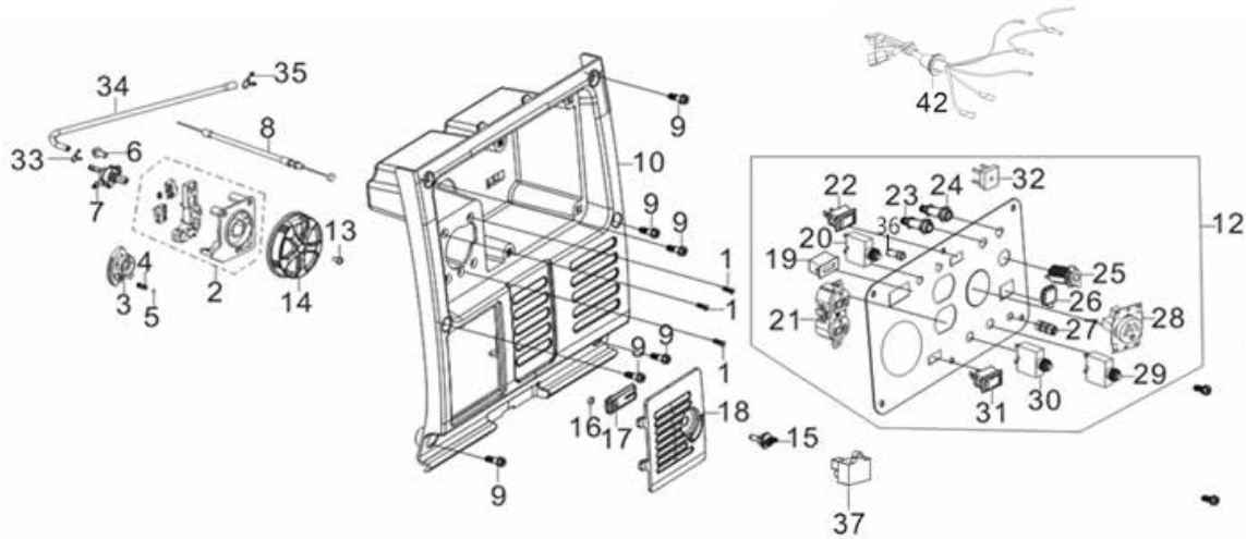
Fig. 14 - Control Panel Assembly
