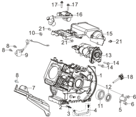
Fig. 1 - Crankcase Assembly
