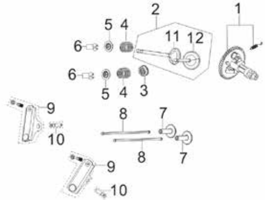
Fig. 6 - Valve Train & Camshaft Subassembly
