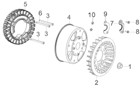
Fig. 9 - Rotor/Stator Assembly
