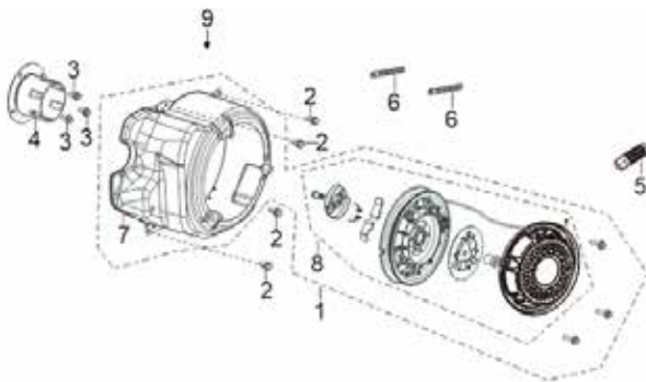
Fig. 7 - Recoil Starter
