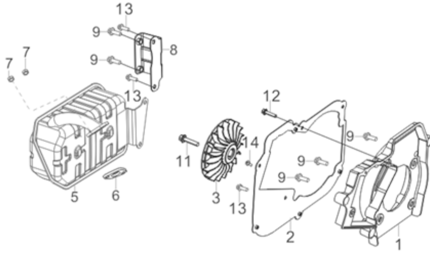
Fig. 11 - Muffler Assembly
