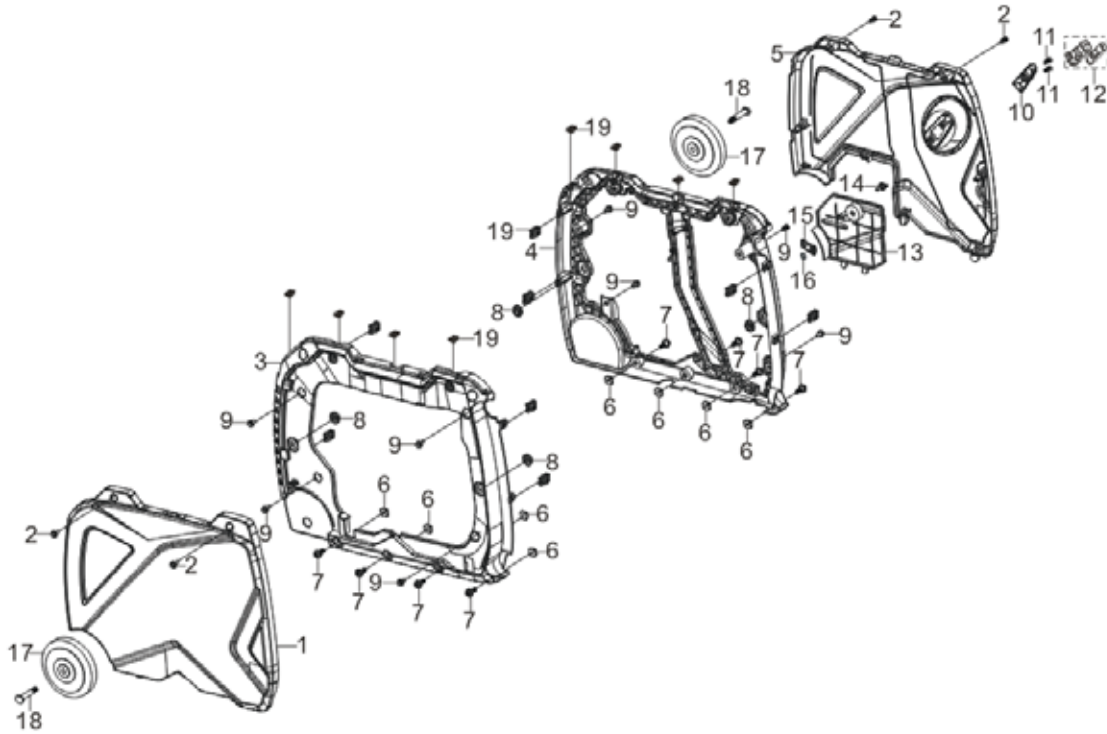
Fig. 16 - Side Covers
