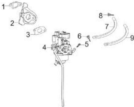
Fig. 8 - Carburetor Assembly
