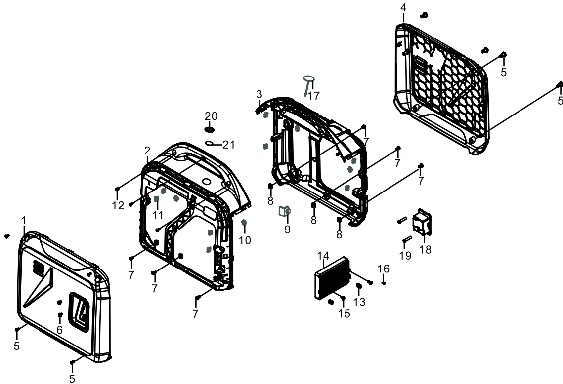
FIG. 11 - HOUSING
