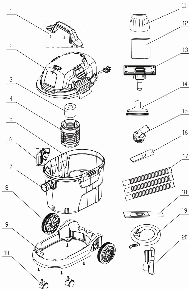
VHB307WM Parts List
