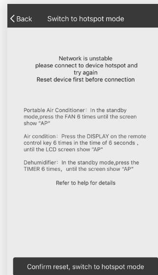
Connection Failed
