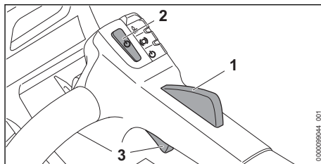
Trigger Switch Lockout (1), Retaining Button (2) and Trigger Switch (3)
