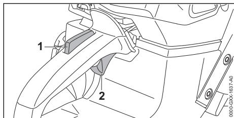
Throttle Trigger Lockout (1) and Throttle Trigger (2)
