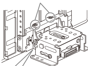
Pre-installed screws
