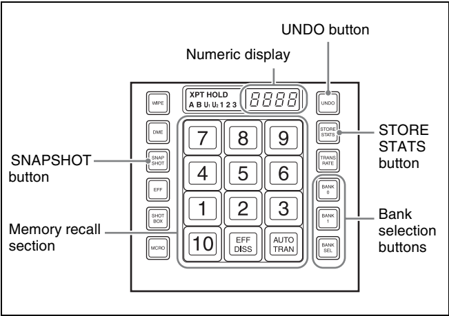
Flexi Pad control block (standard type)
