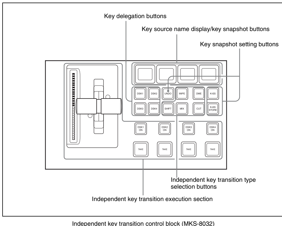
Independent key transition control block (MKS-8032)
