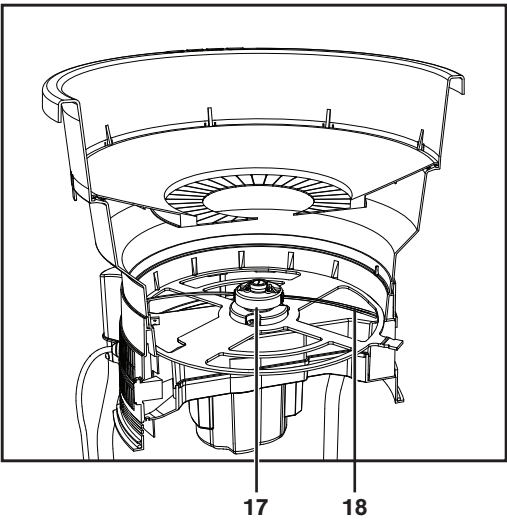
CUTAWAY VIEW
