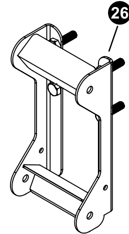
BACKBOARD BOX 1A-7905-20 (QTY. 1)
