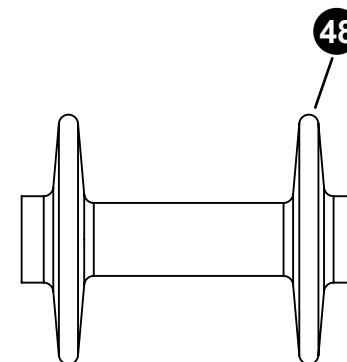
ACTUATOR ROLLER 3M-9035-00 (QTY. 1)
