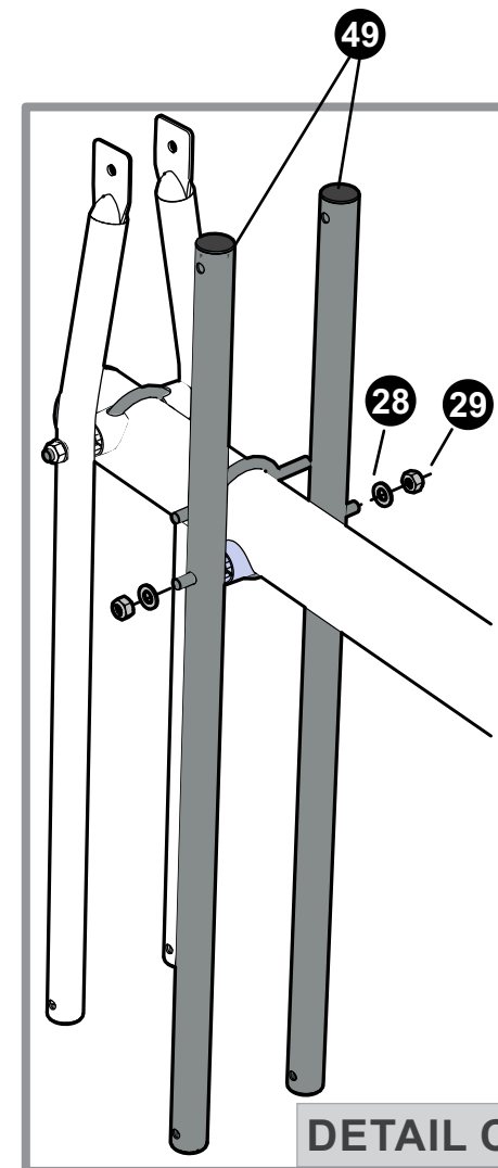
HEX LOCK NUT M12-1.75 2B-6805-00 (QTY. 4)
