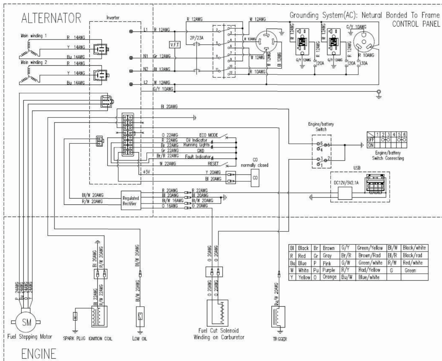
WIRING DIAGRAM
