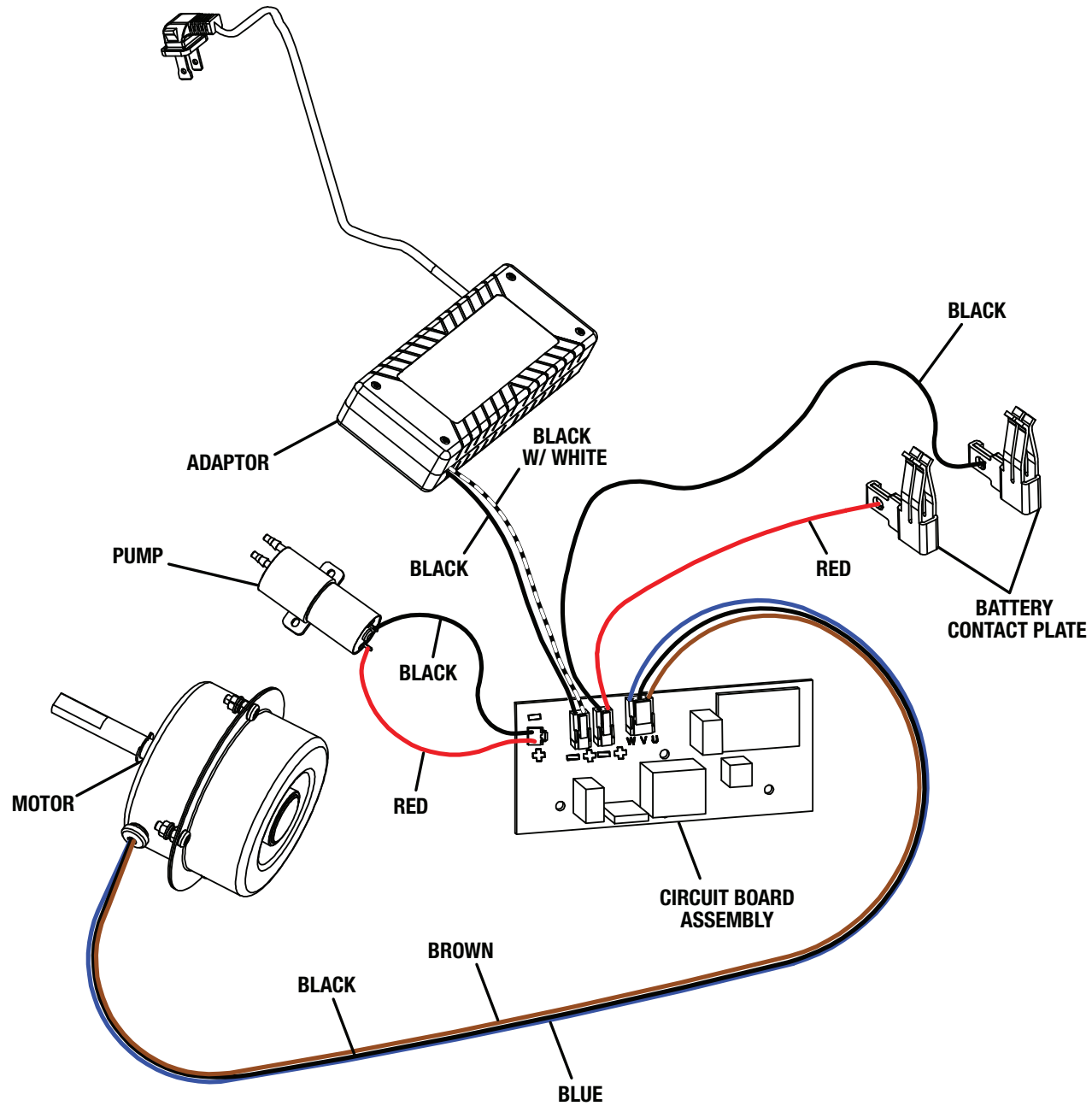
WIRING DIAGRAM
