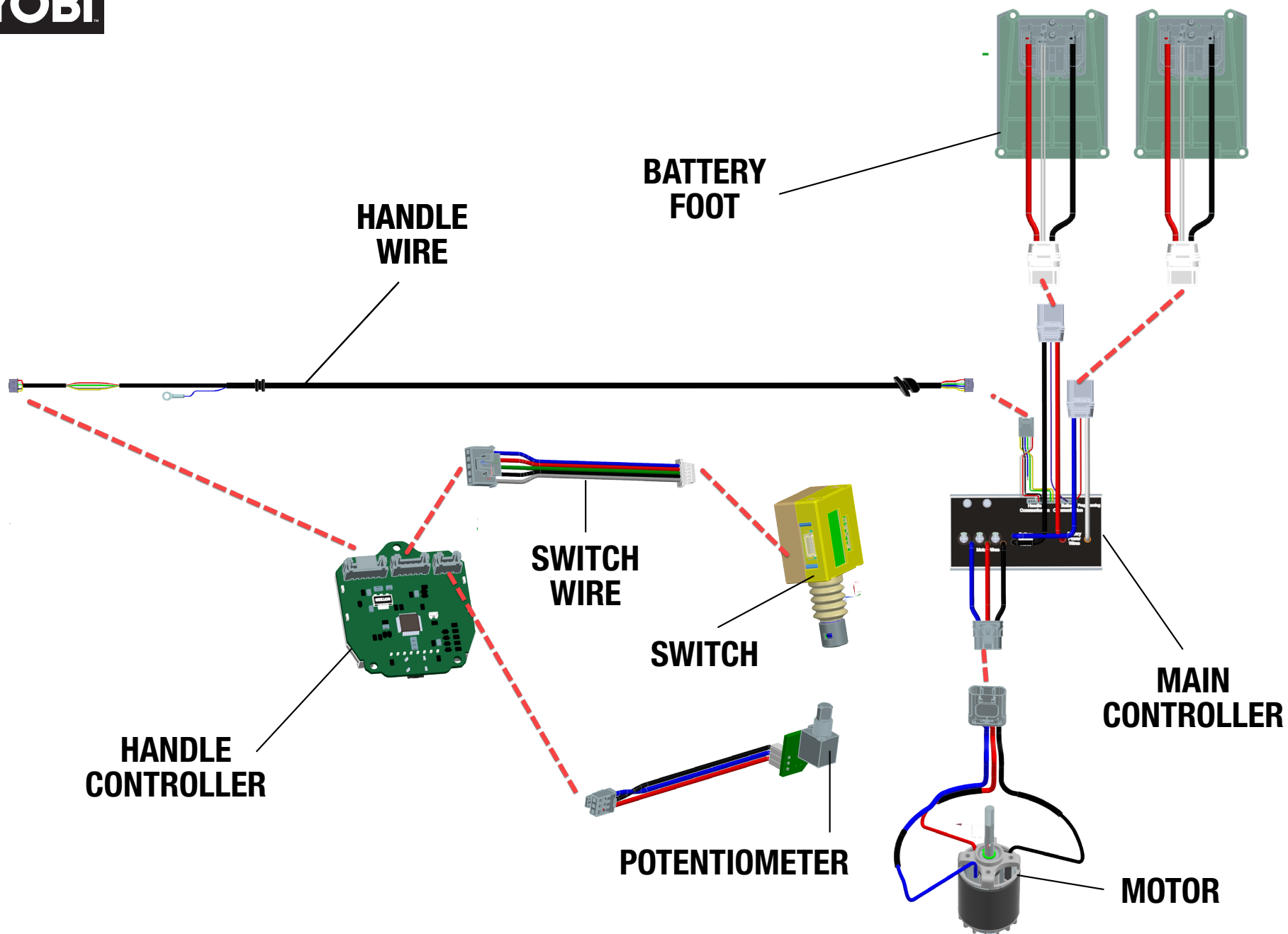
WIRING DIAGRAM
