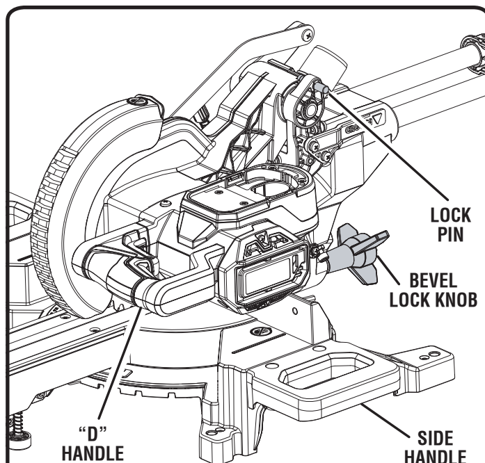
SAW ARM LOCKED IN DOWN POSITION
