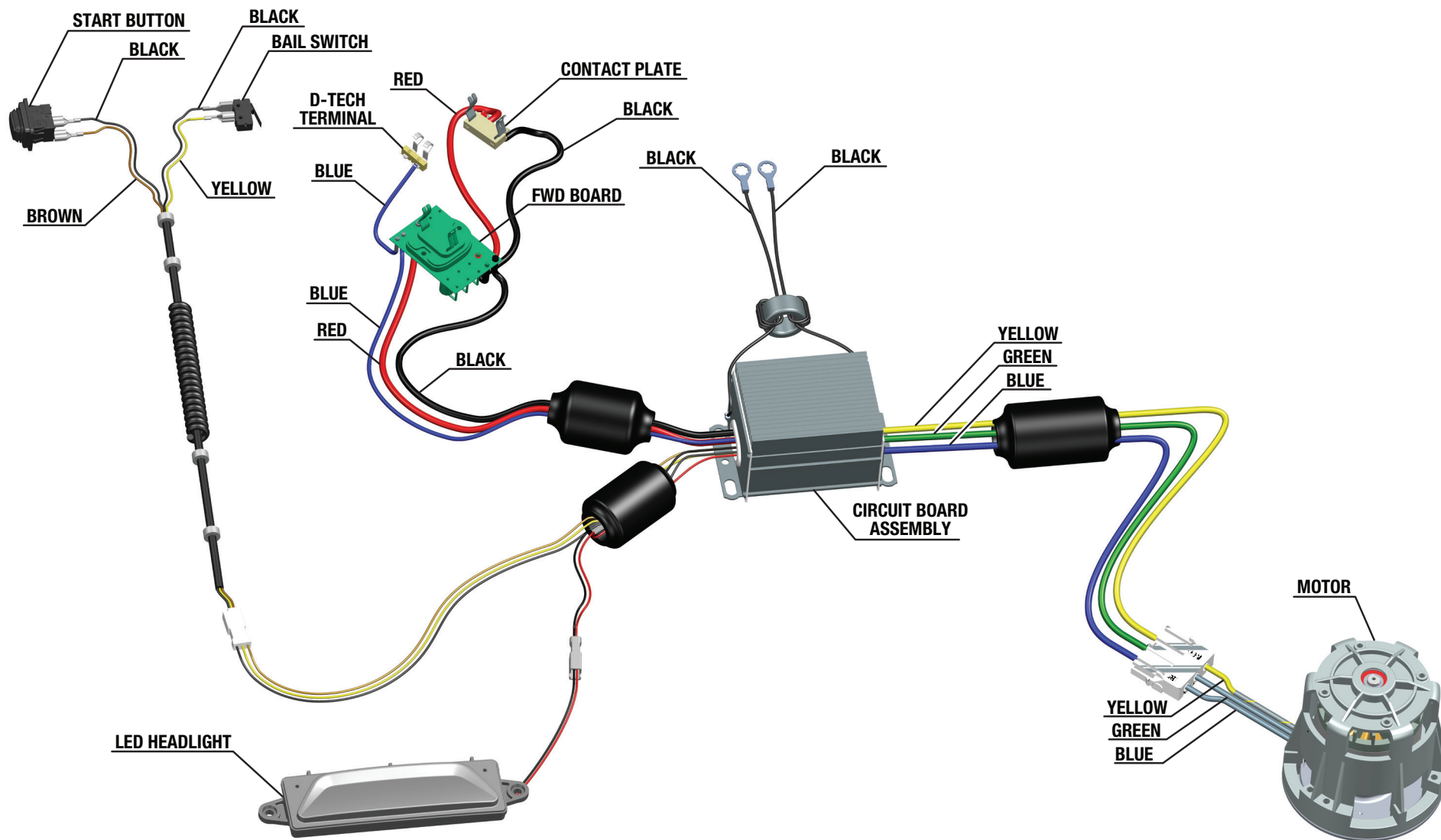
WIRING DIAGRAM
