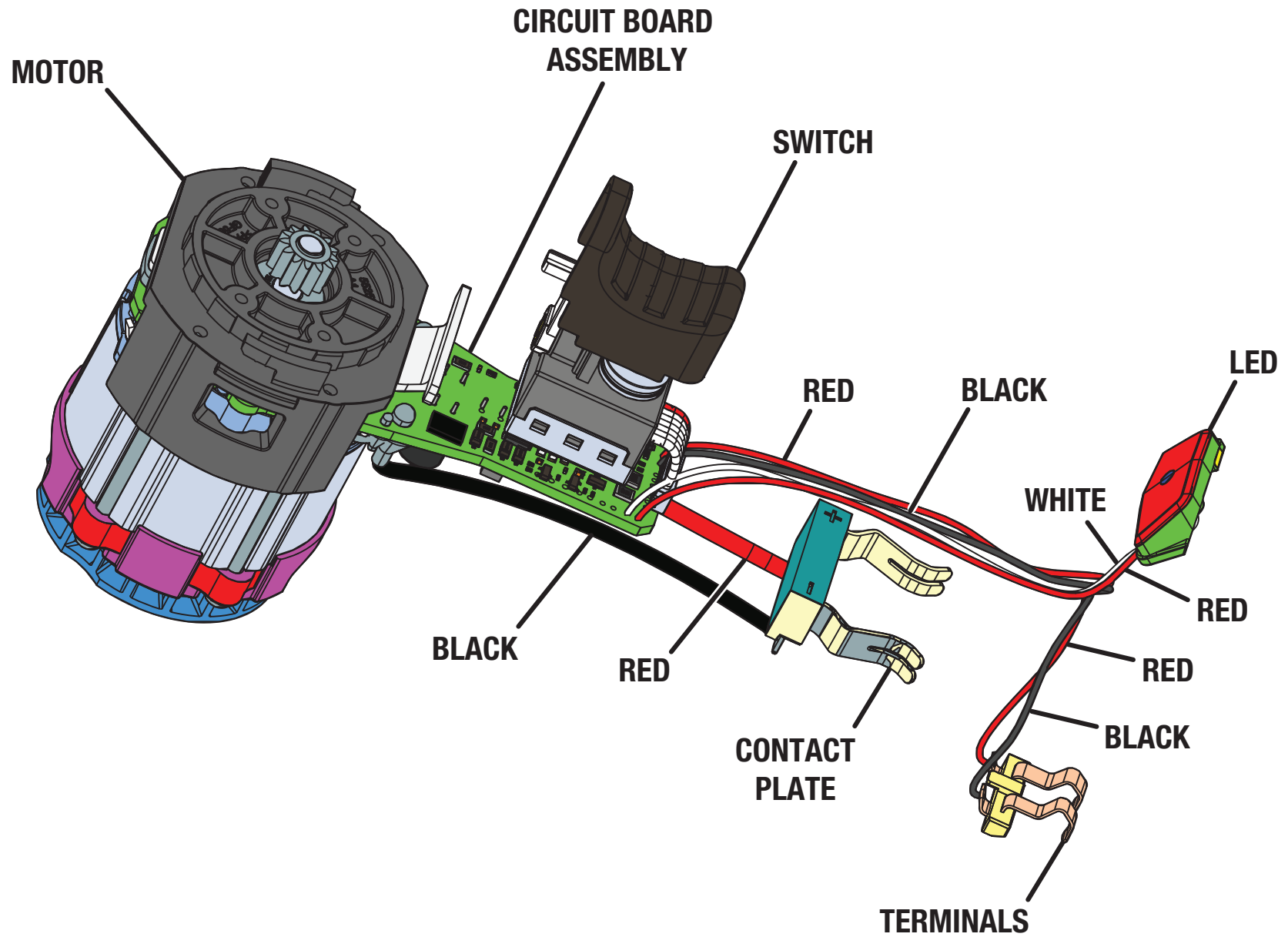
WIRING DIAGRAM
