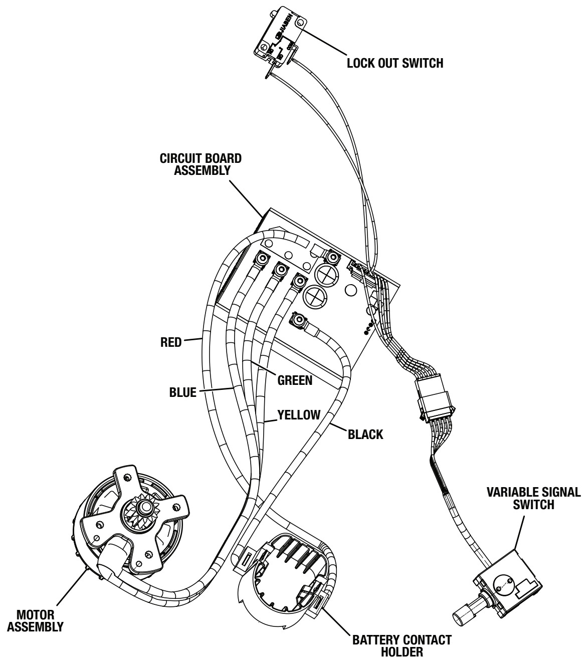
WIRING DIAGRAM
