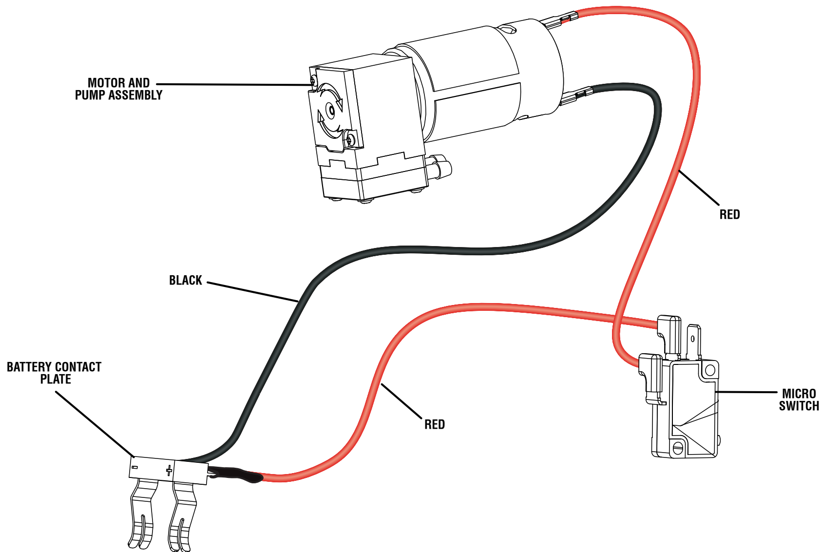
WIRING DIAGRAM
