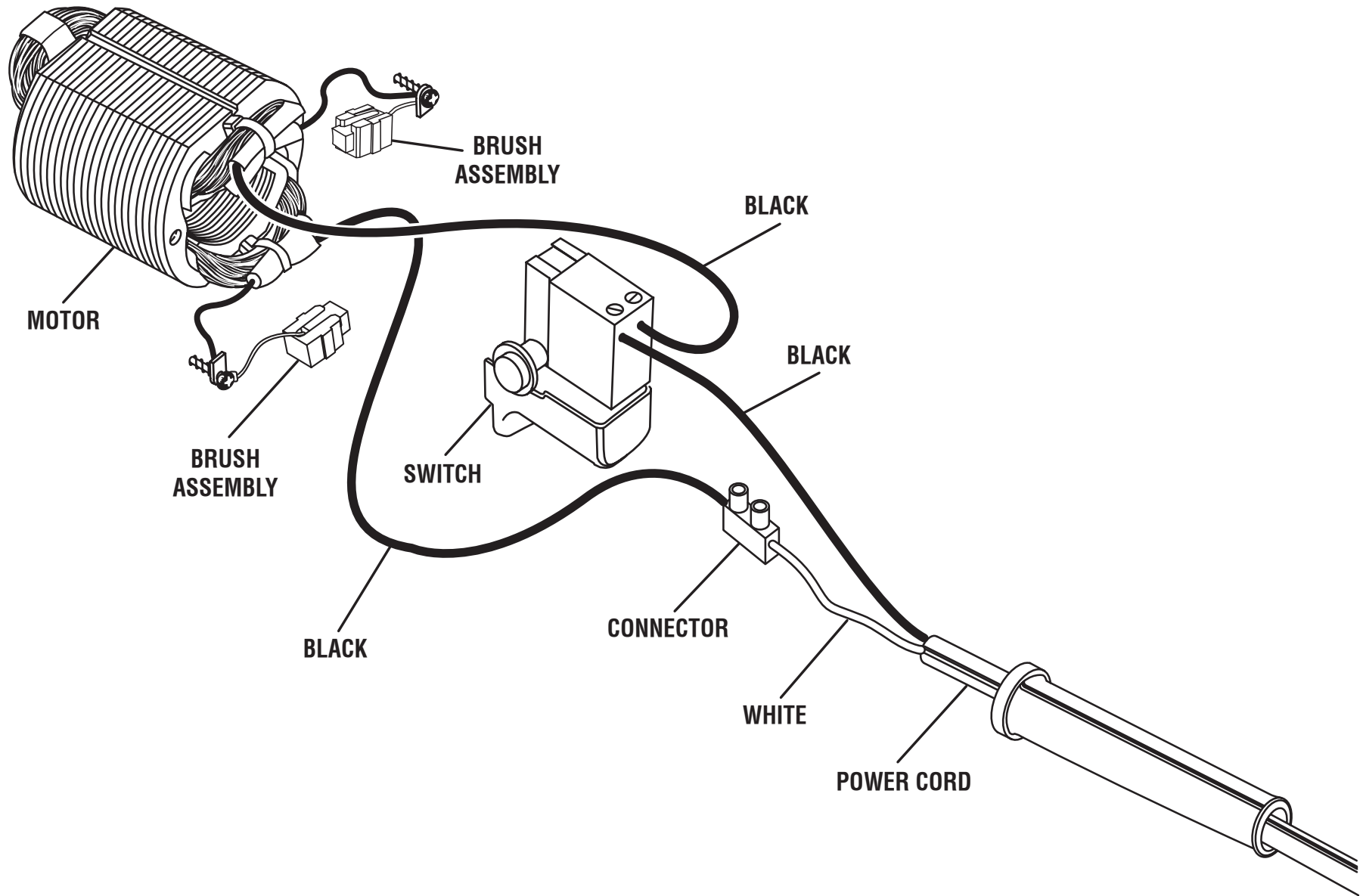
WIRING DIAGRAM
