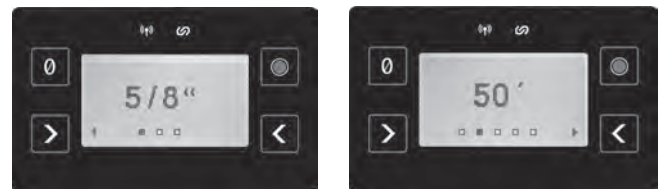
a. Cable Diameter Screen b. Cable Length Screen Figure 11 – Setting Cable Parameters
