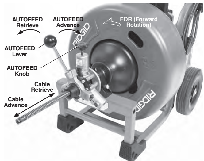
Figure 18 – Cable Movement in FOR (Forward Rotation)
