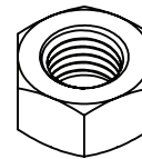
10-0315 X20 M24X3.00, NUT STEP 1A, 2A, 3, 4, 5
