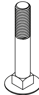
10-0183 X8 M16X2.00, L100, CARRIAGE BOLT STEP 1B, 2B
