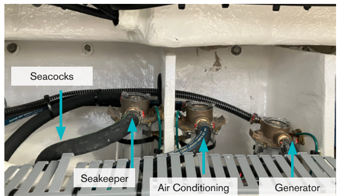
Seacock strainers
