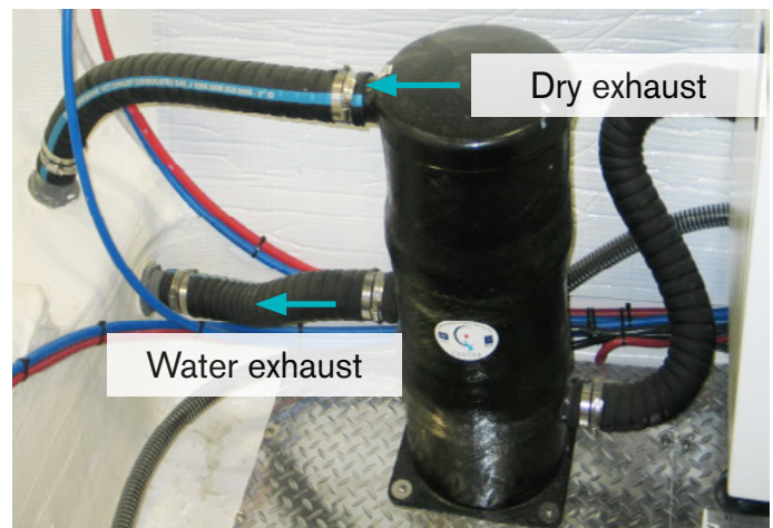
Generator muffler
