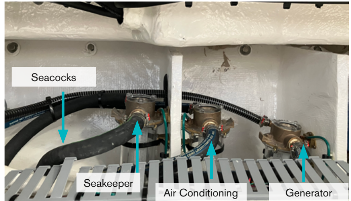
Seacock strainers
