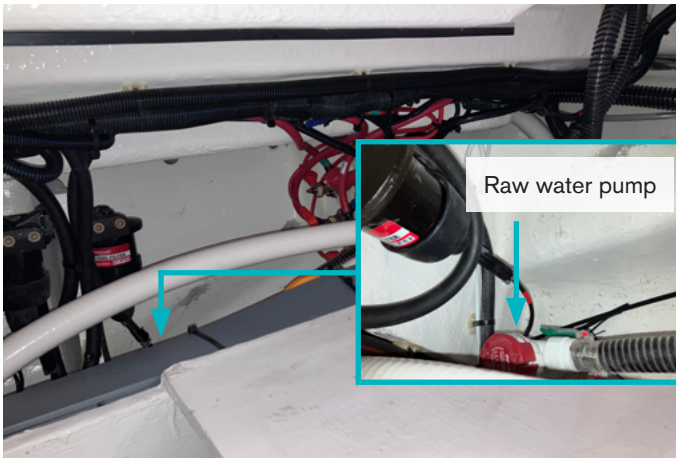
Port seacock and pump
