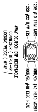
HC2 - HARNESS CONNECTION #2
