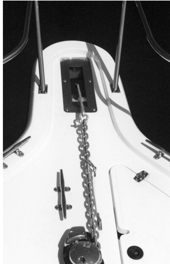
Anchor Chain Properly Secured for Travel
