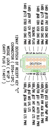
HC3 - HARNESS CONNECT #3 (GREEN)
