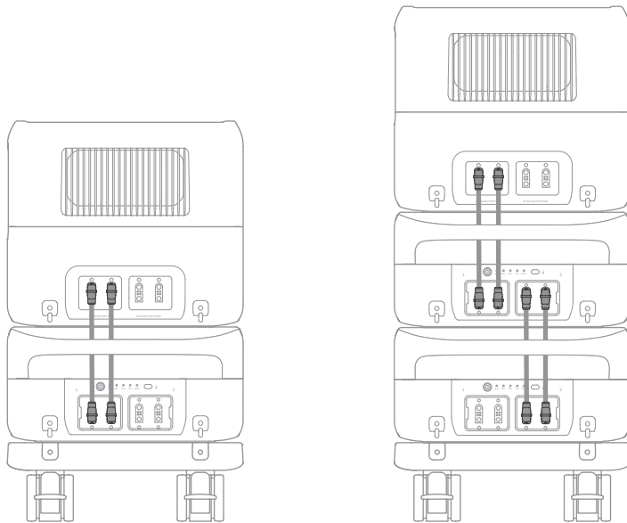
Cascade Connection for 1 Battery Unit
