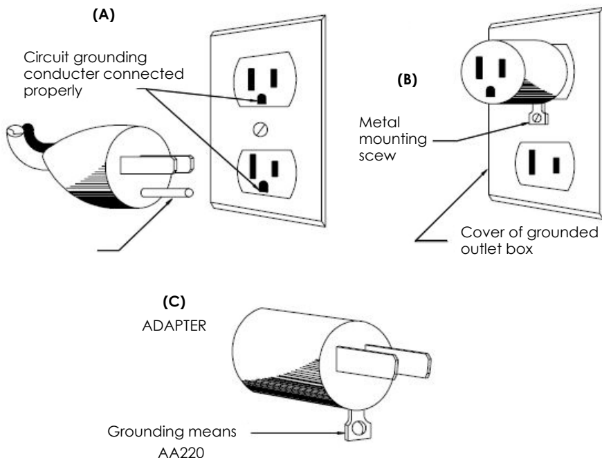
FIGURE 73.1 Grounding Methods
