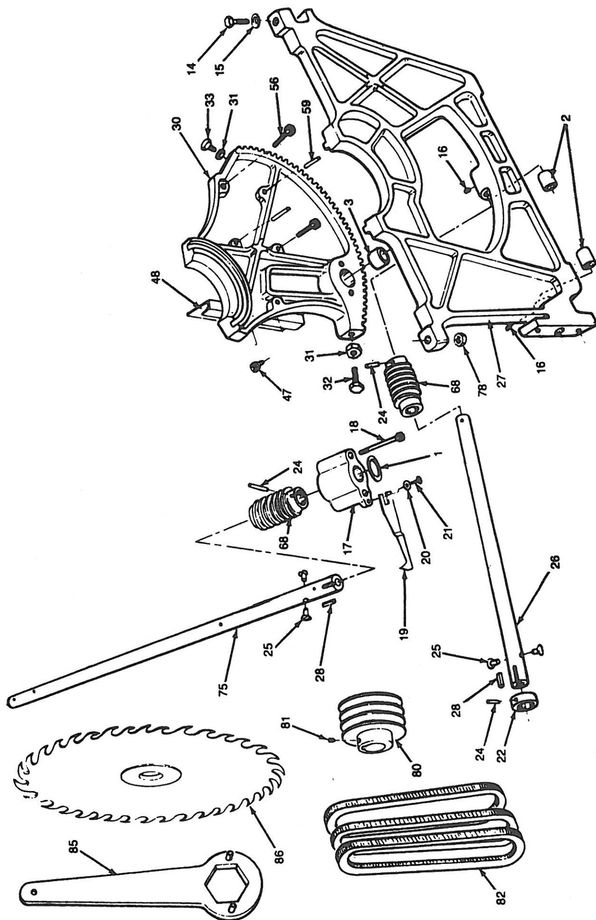
Figure 3 — Replacement Parts Illustration for Main Mechanism
