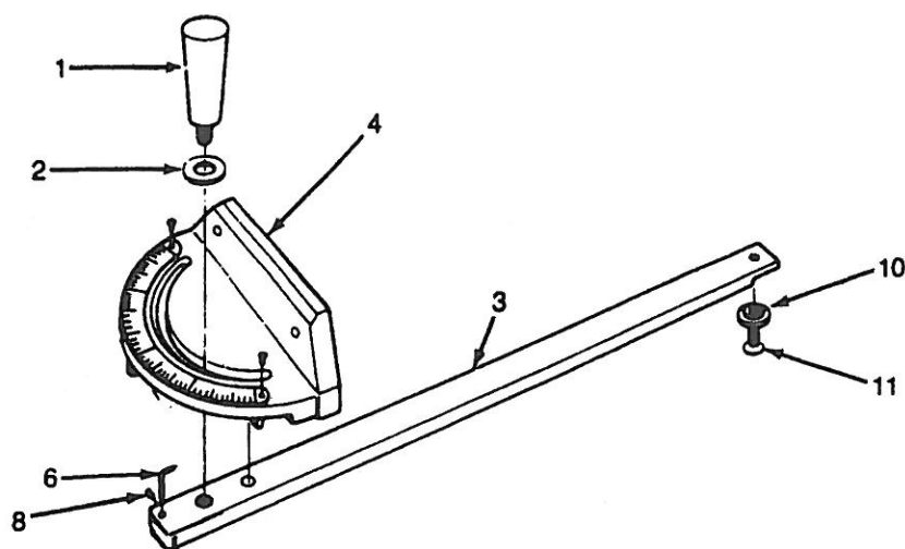
Figure 1 — Replacement Parts Illustration for Miter Gauge
