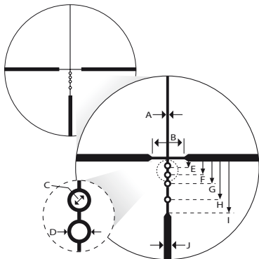
BDC 150 reticle
