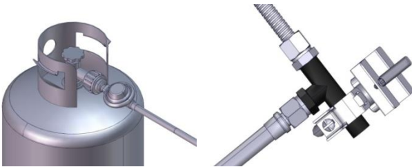
Propane tank: height = 456mm, diameter = 320mm
