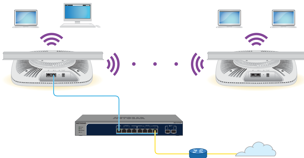
Figure 10. WiFi bridge configuration between two access points in the 5 GHz radio band
