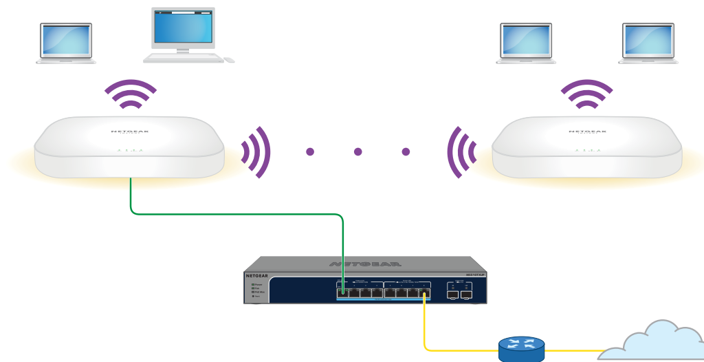
Figure 8. WiFi bridge configuration between two access points in the 5 GHz radio band
