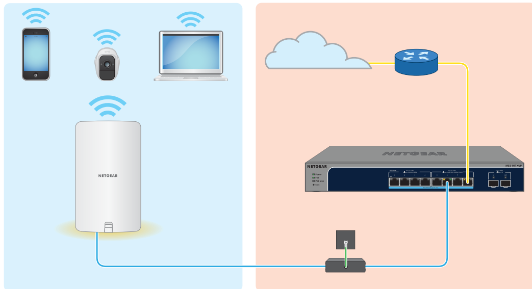
Figure 4. Set up the access point with a PoE+ connection to your network
