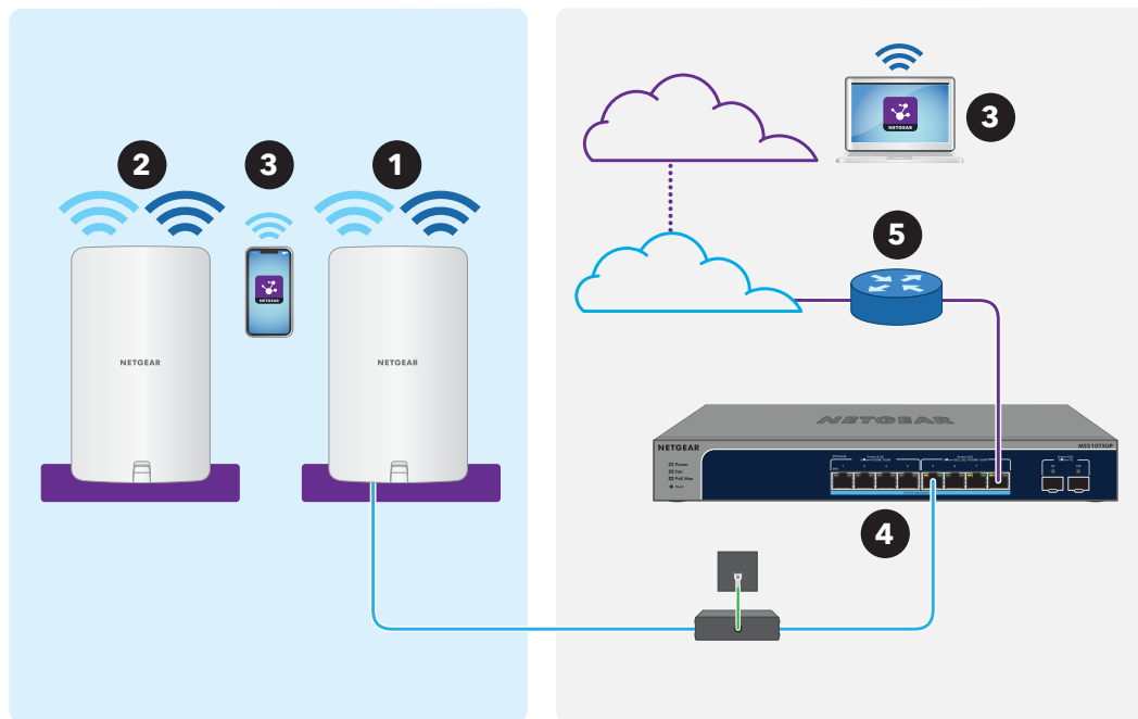
Figure 7. Connect the node to a wired root
