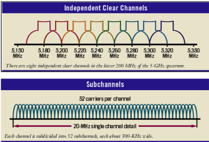
Figure B-3: IEEE 802.11a Channel Allocations
