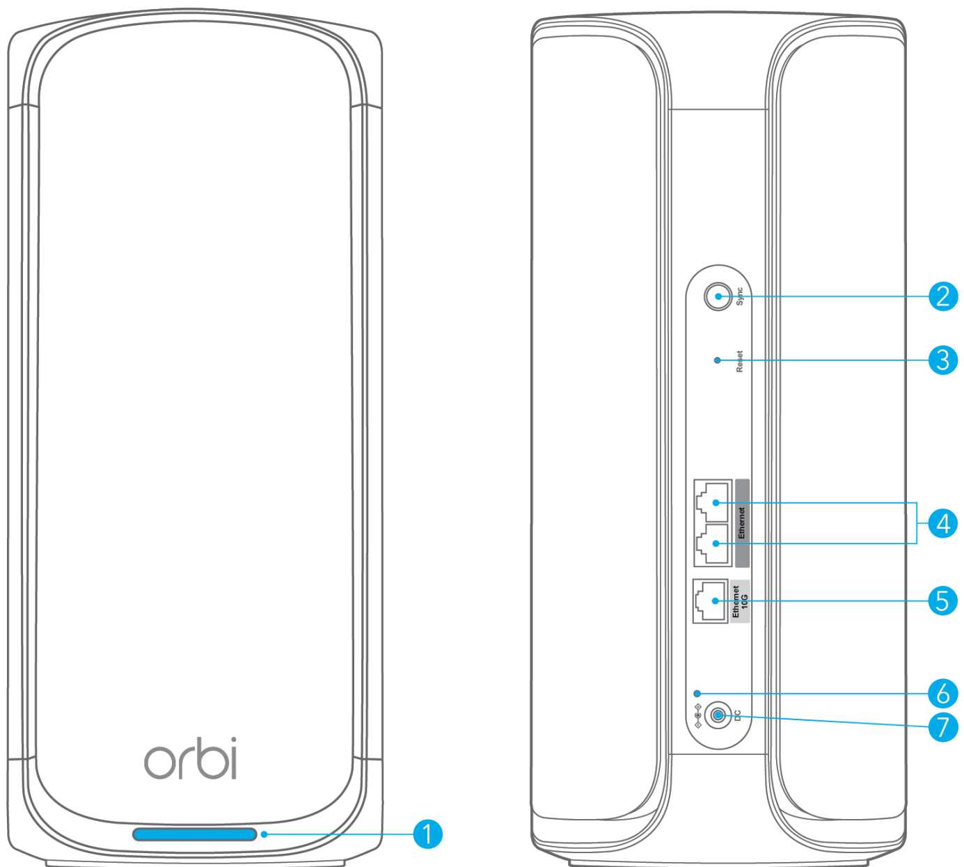
Figure 2. Orbi satellite front (left figure) and back (right figure) views
