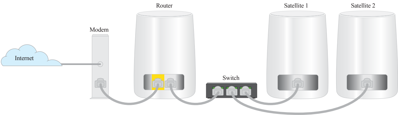
Figure 6. Ethernet backhaul connection using a switch
