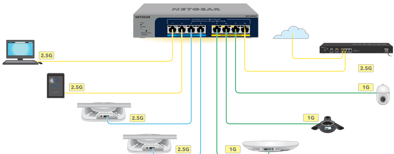
Figure 1. Example connections
