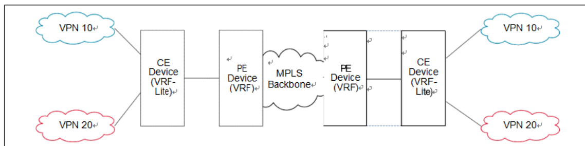
Figure 7-10: VRF Scenarios
