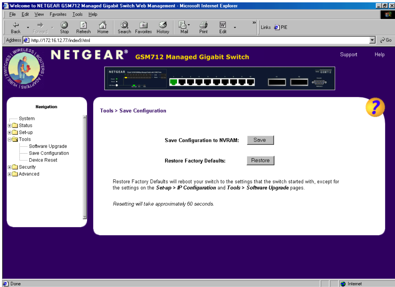
Figure 7-13: Save Configuration
