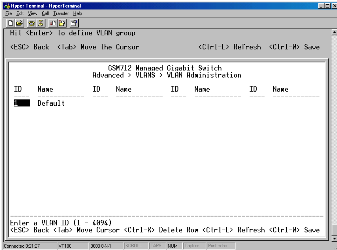
Figure 6-18: VLAN Administration
