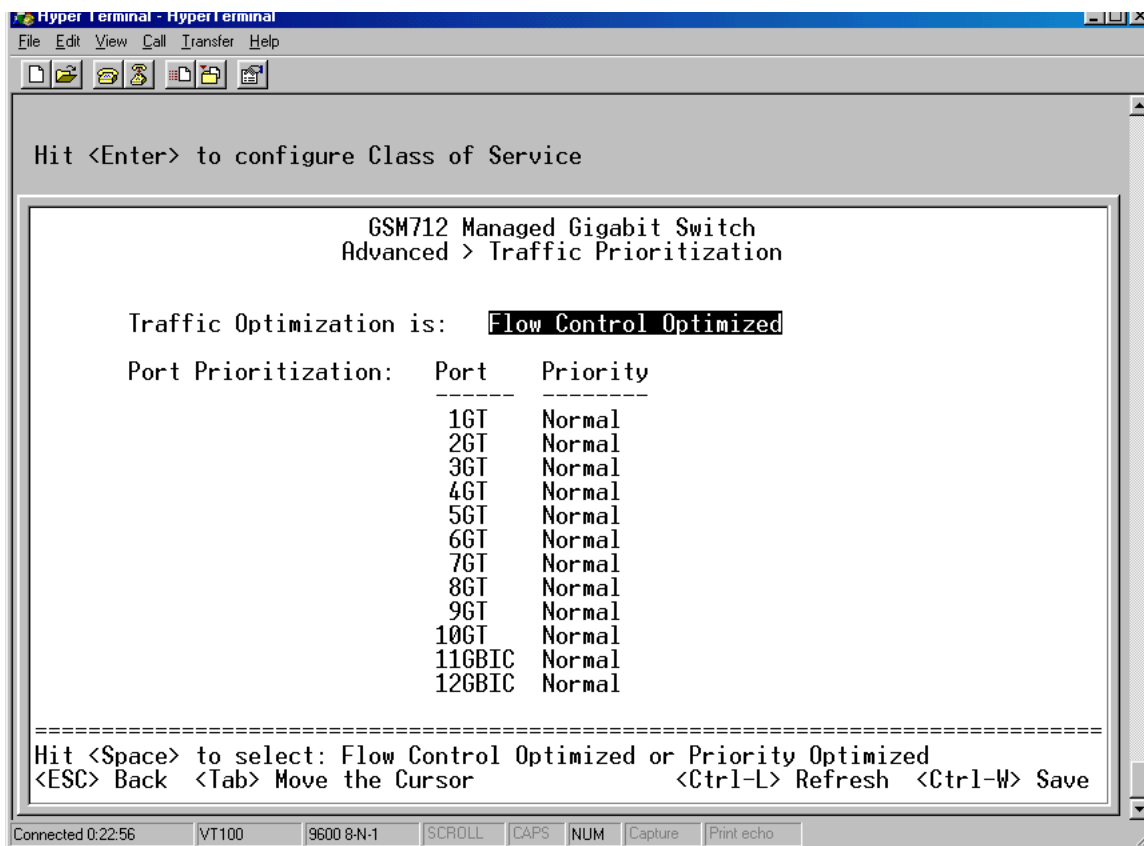
Figure 6-16: Traffic Prioritization
