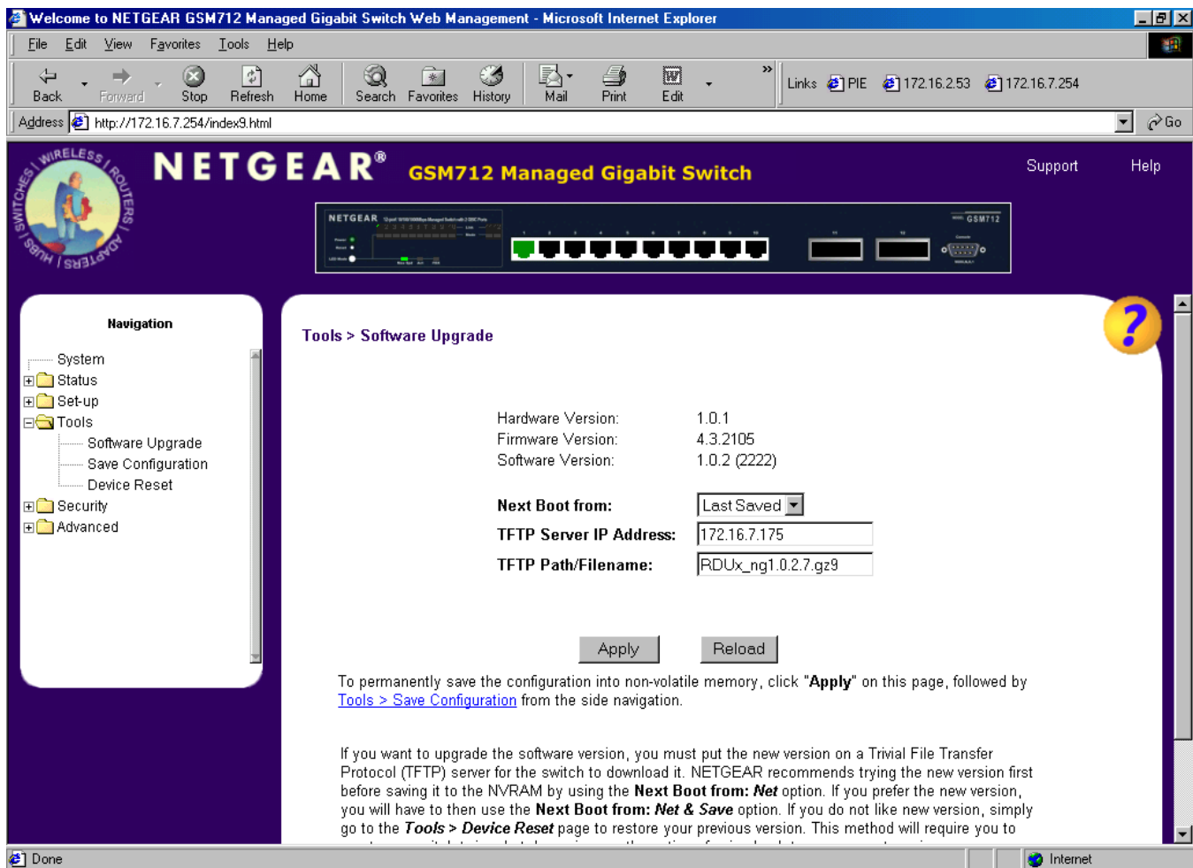
Figure 7-12: Software Upgrade
