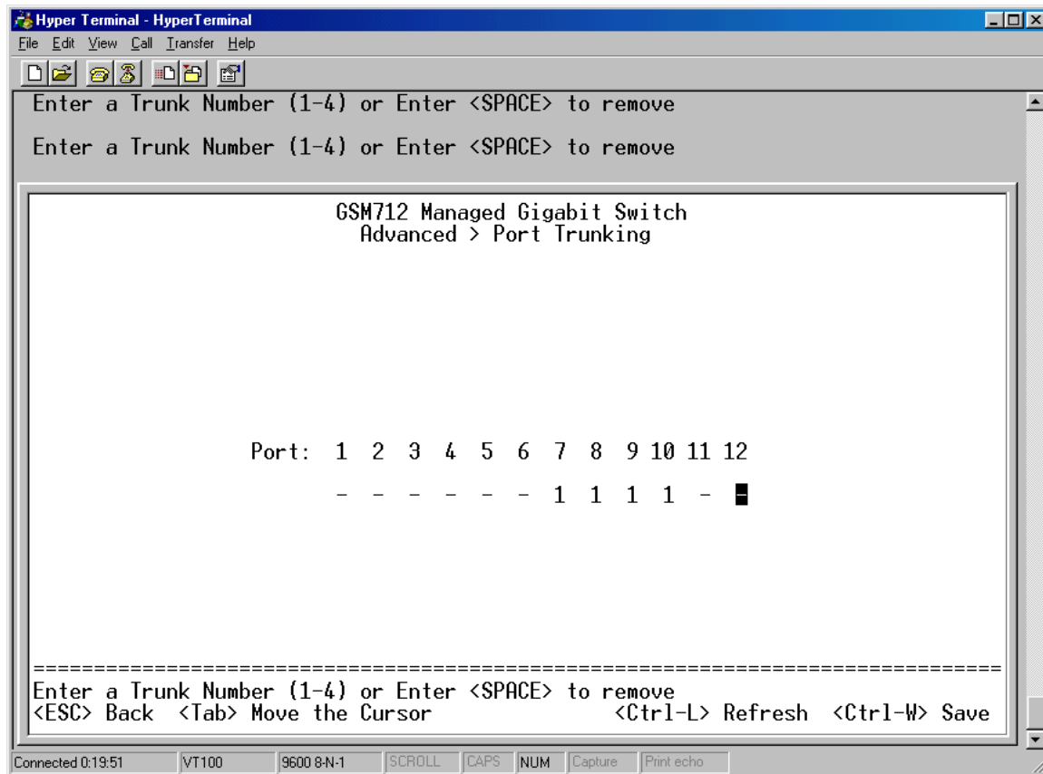
Figure 6-14: Port Trunking
