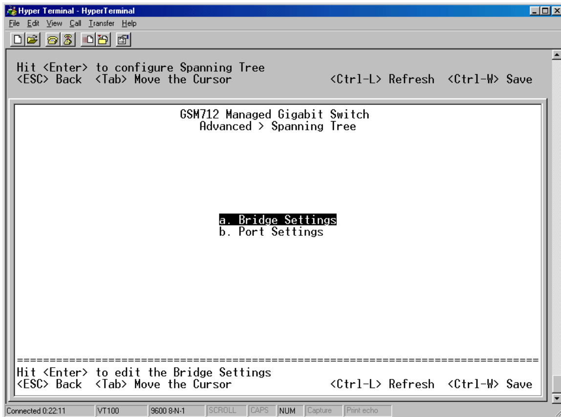
Figure 6-21: Spanning Tree
