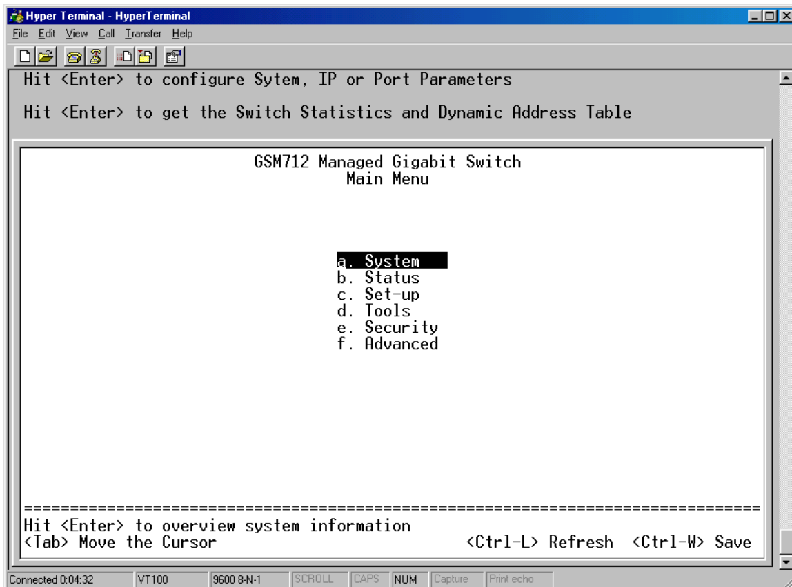
Figure 6-3: Main Menu
