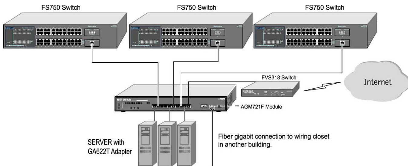
Figure 3-2. Example of Backbone Switching
