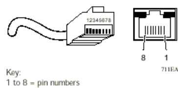
Figure E-1. RJ-45 Plug and RJ-45 Connector with Built-in LEDs
