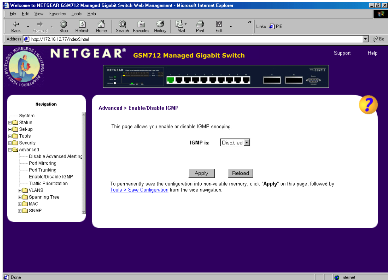
Figure 7-19: IGMP
