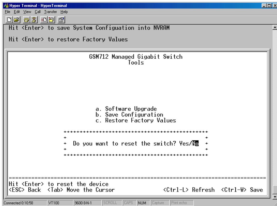
Figure 6-11: Reset
