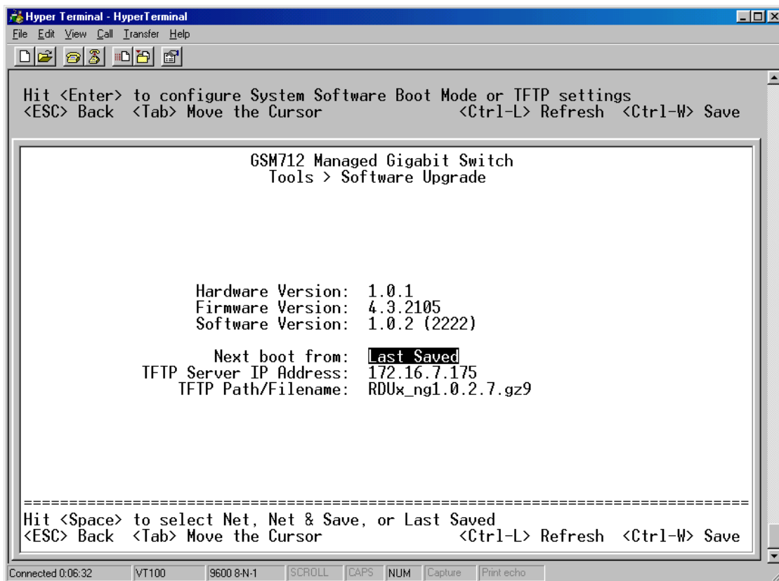
Figure 6-9: Software Update
