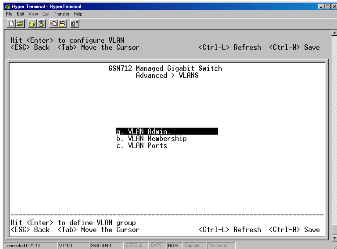
Figure 6-17: VLANs Set-up
