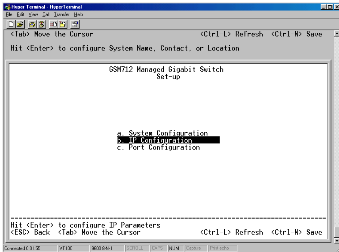
Figure 4-5 Set-Up
