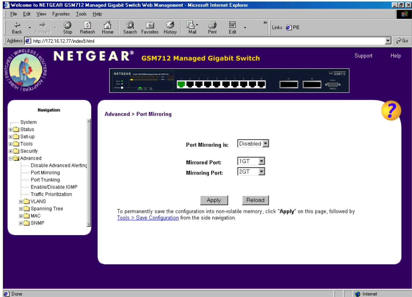
Figure 7-17: Port Mirroring
