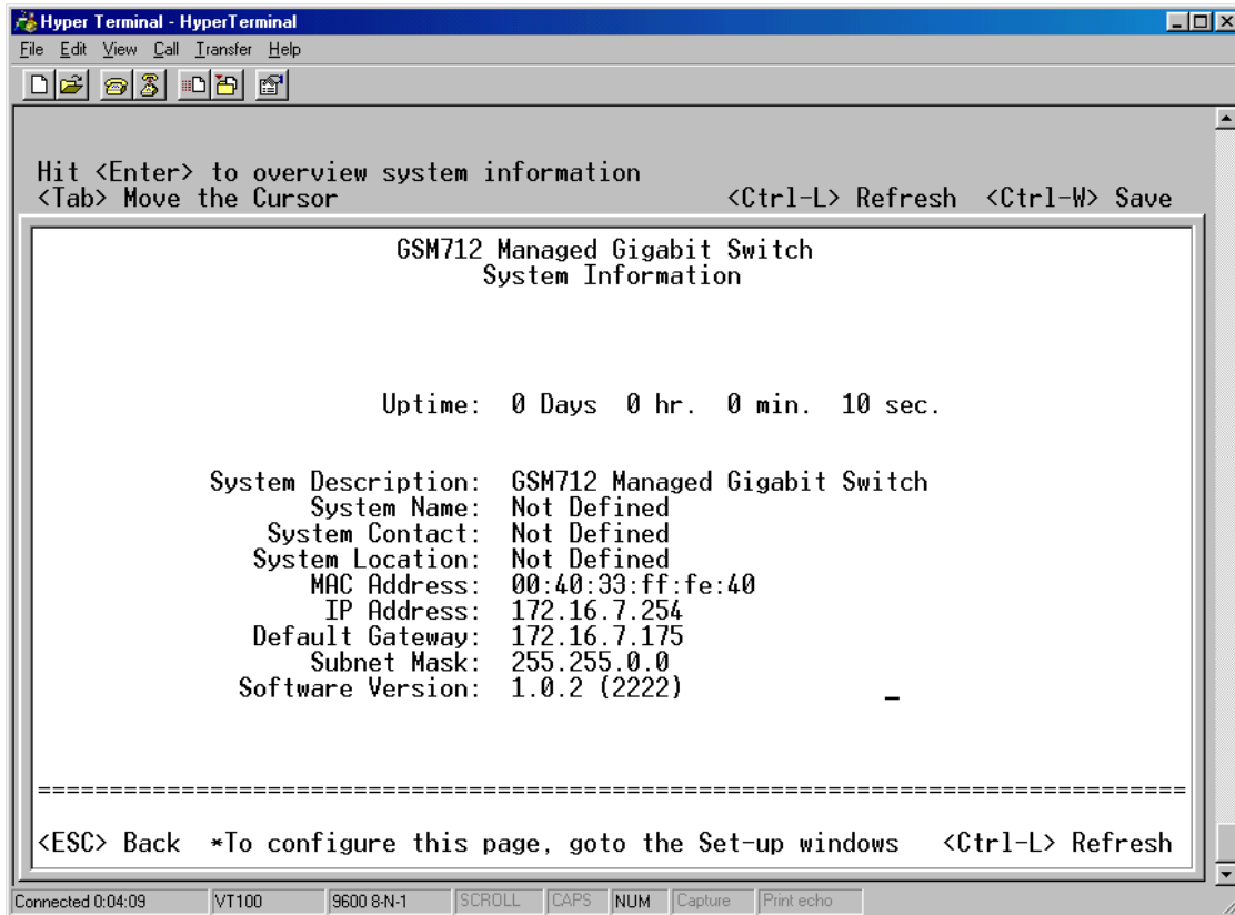
Figure 6-4: System Information
