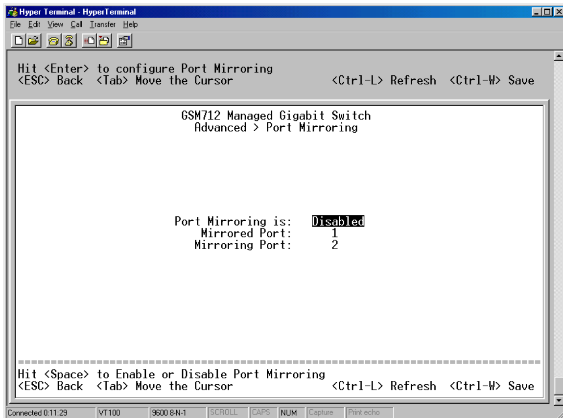
Figure 6-13: Port Mirroring
