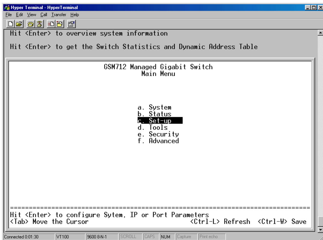
Figure 4-4 Main Menu
