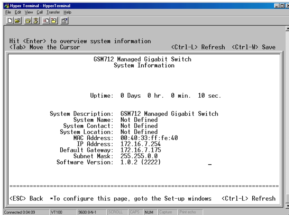
Figure 4-3 System Information
