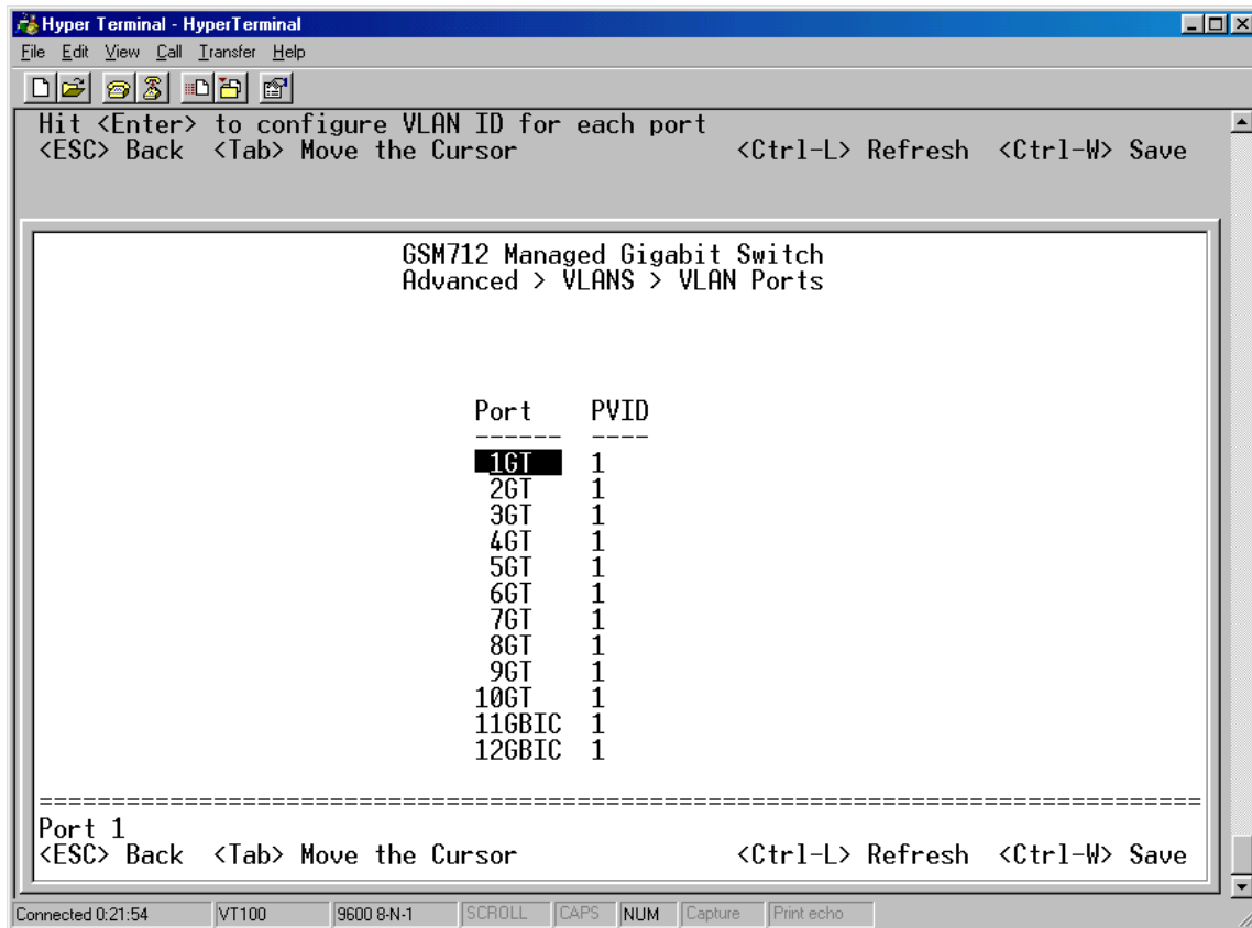
Figure 6-20: VLAN Ports
