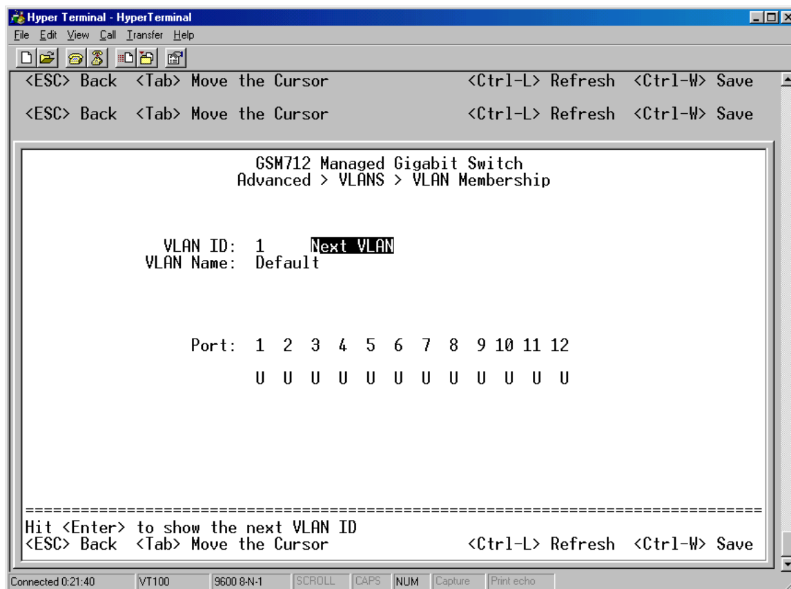
Figure 6-19: VLAN Membership
