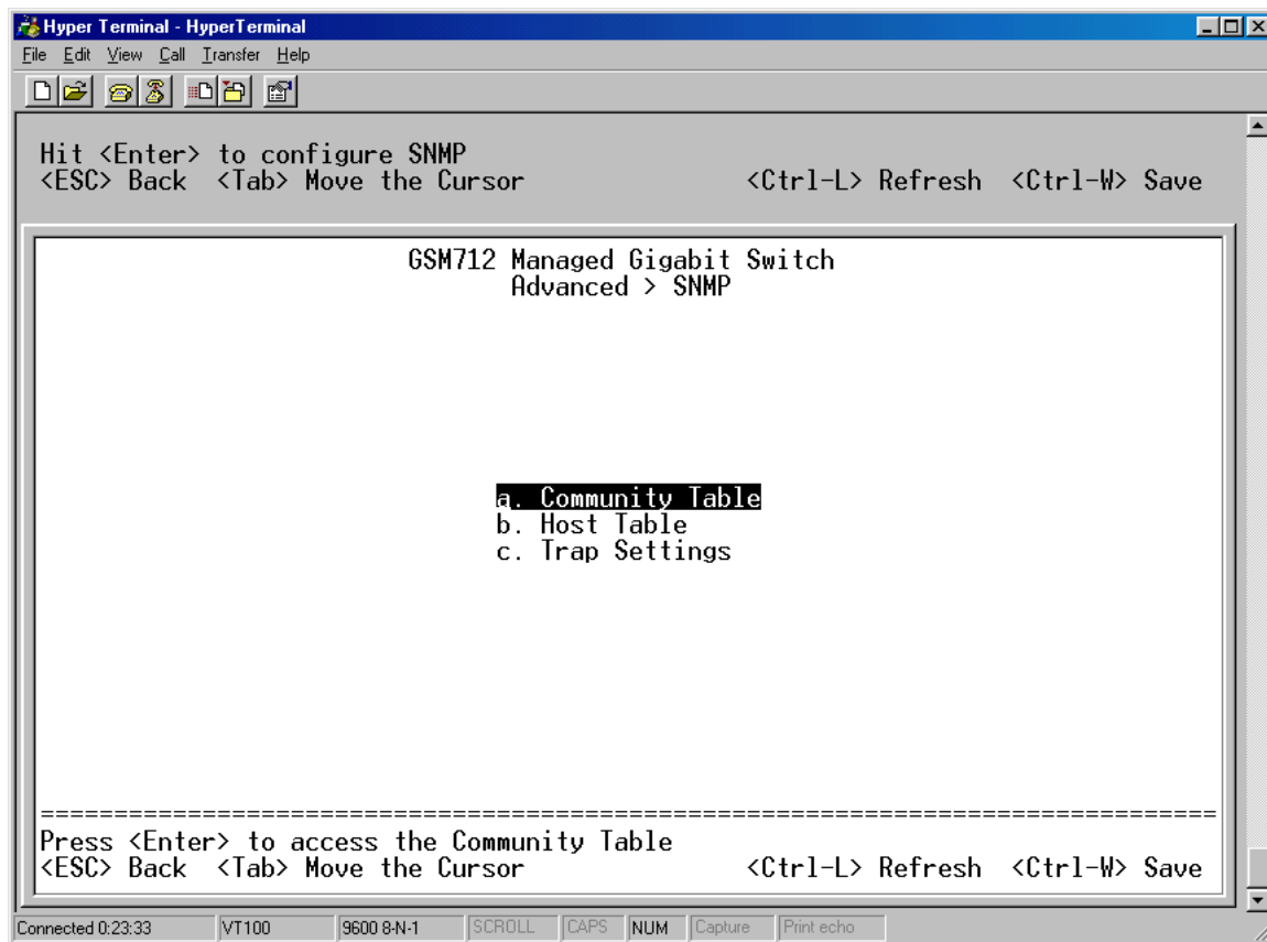
Figure 6-27: SNMP Management
