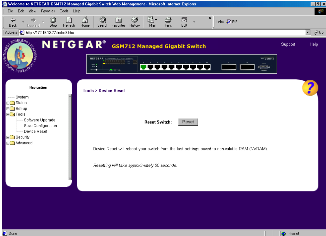
Figure 7-14: Device Reset
