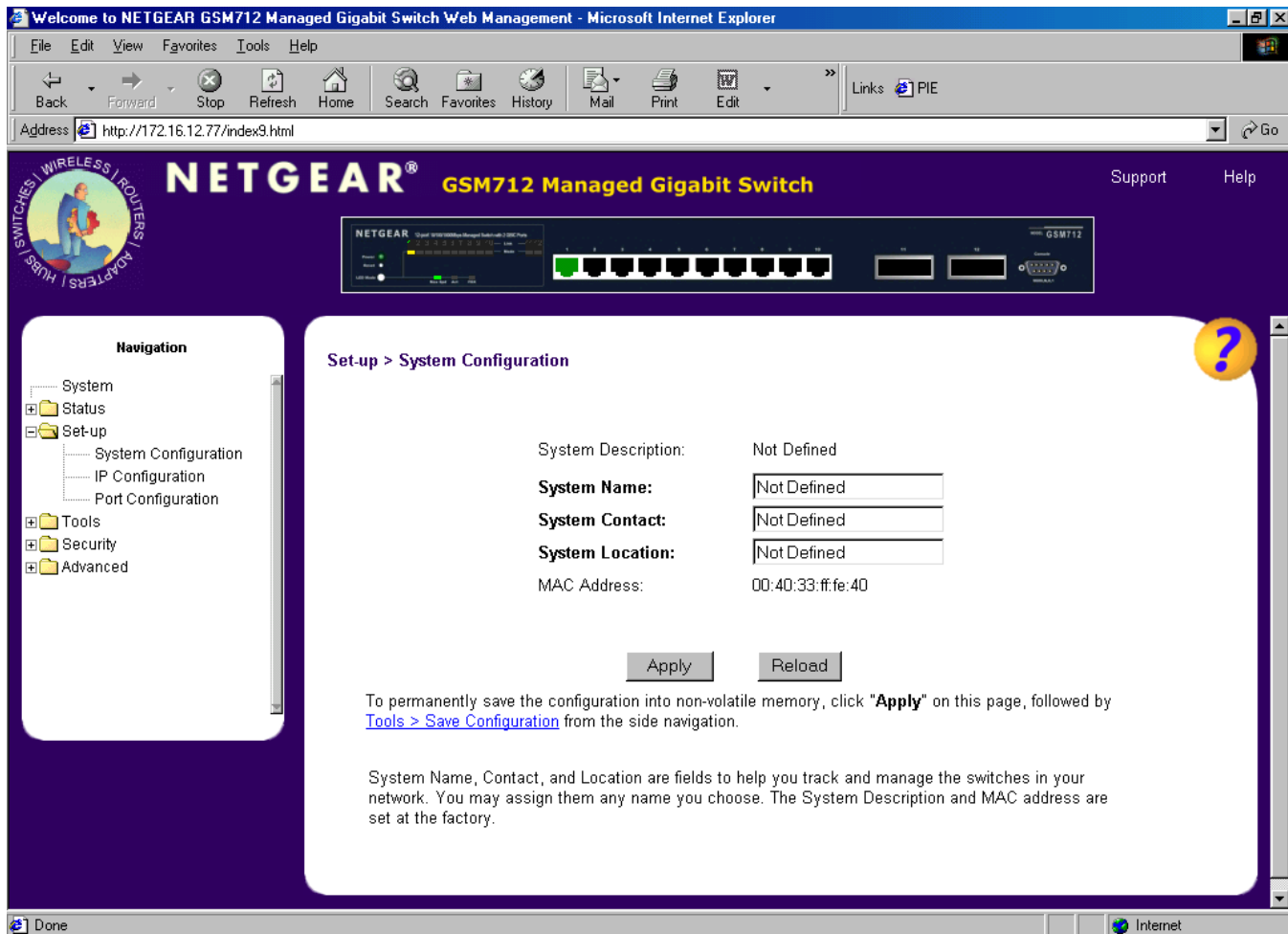
Figure 7-9: System Configuration
