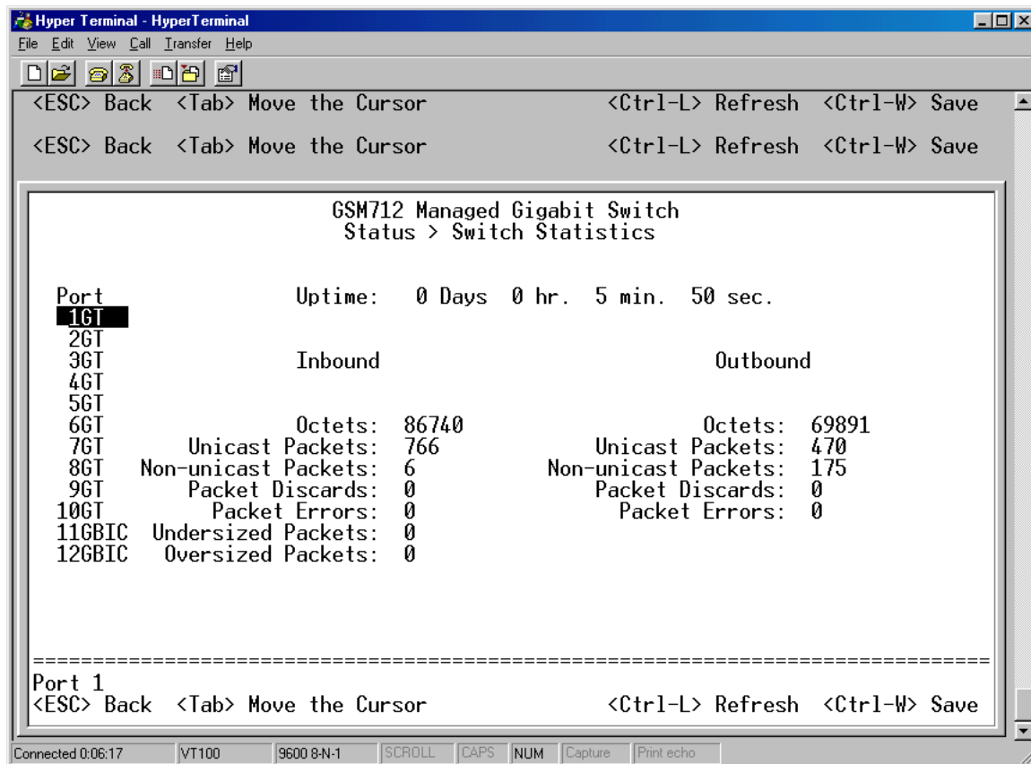
Figure 6-5: Switch Statistics
