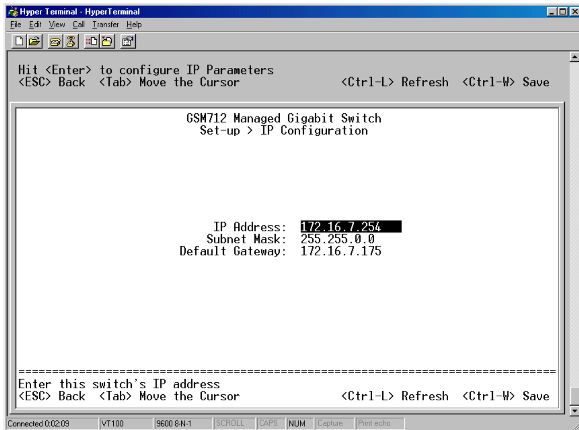
Figure 4-6 IP Configuration
