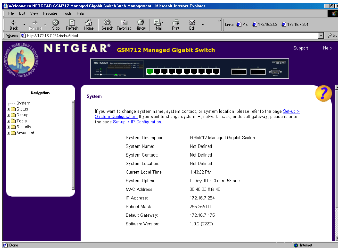
Figure 7-3: System
