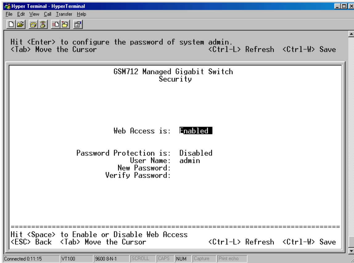
Figure 6-12: Security
