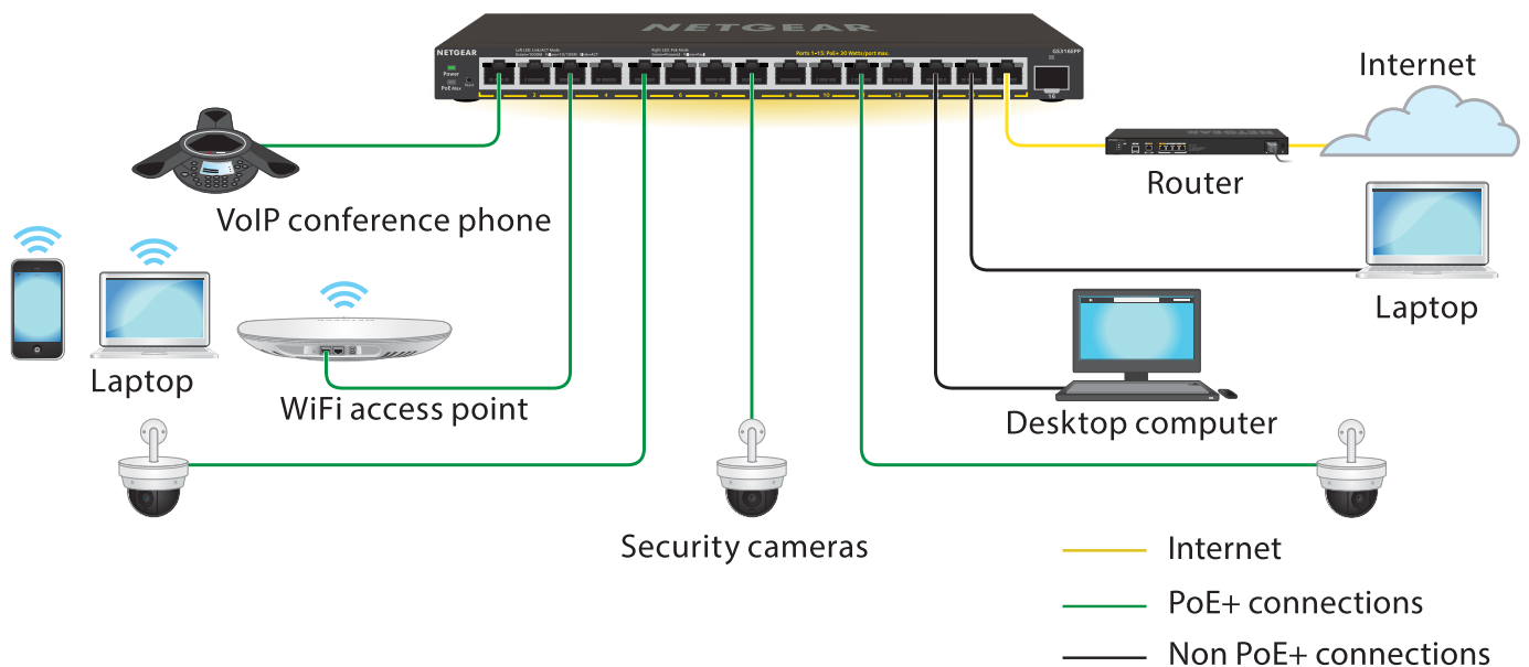
Figure 1. Example connections
