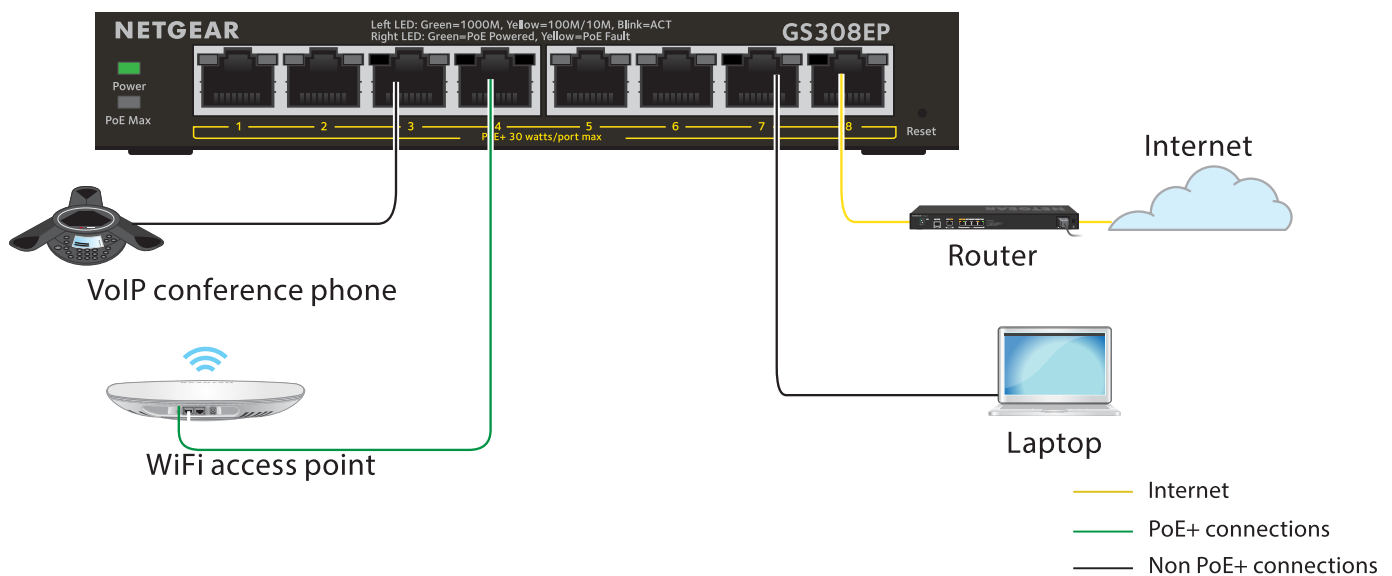
Figure 1. Example connections
