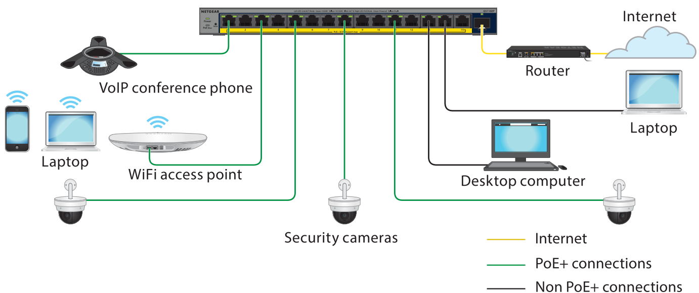
Figure 1. Example connections
