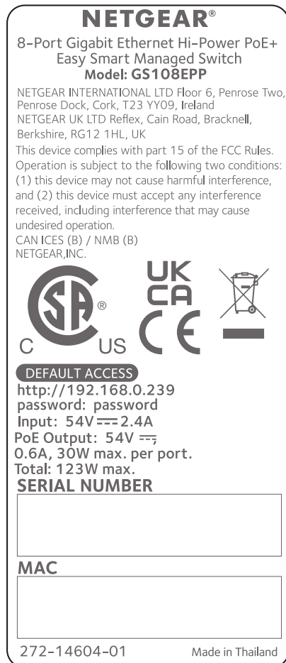
Figure 4. Model GS108EPP
