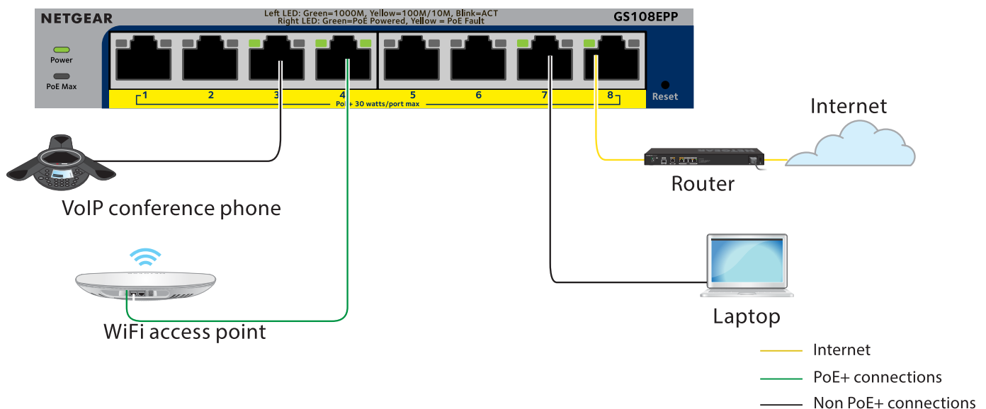
Figure 5. Example connections
