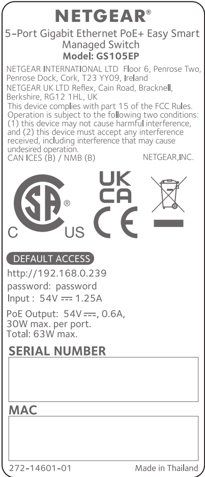
Figure 1. Model GS105EP
