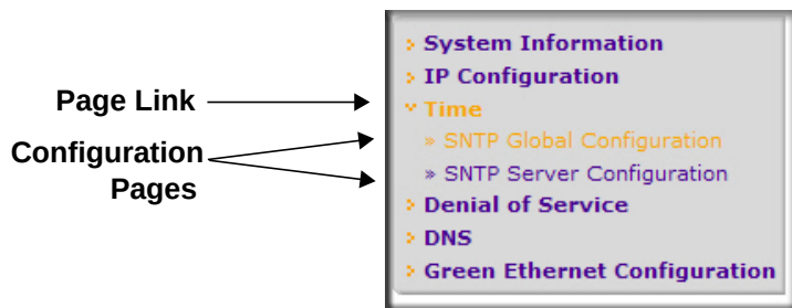
Figure 4. Menu Hierarchy
