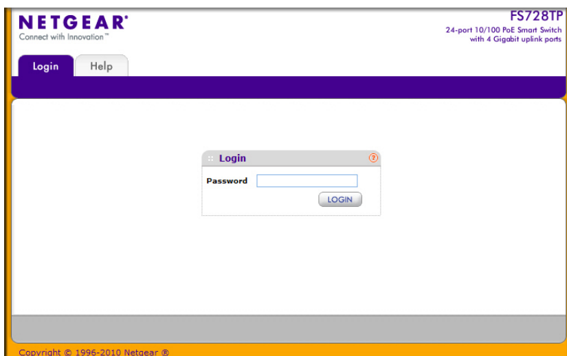
Figure 2. Login Screen
