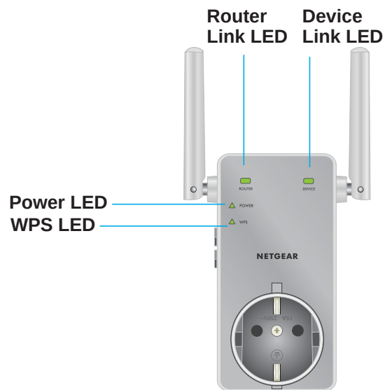
Figure 1. Front panel LEDs
