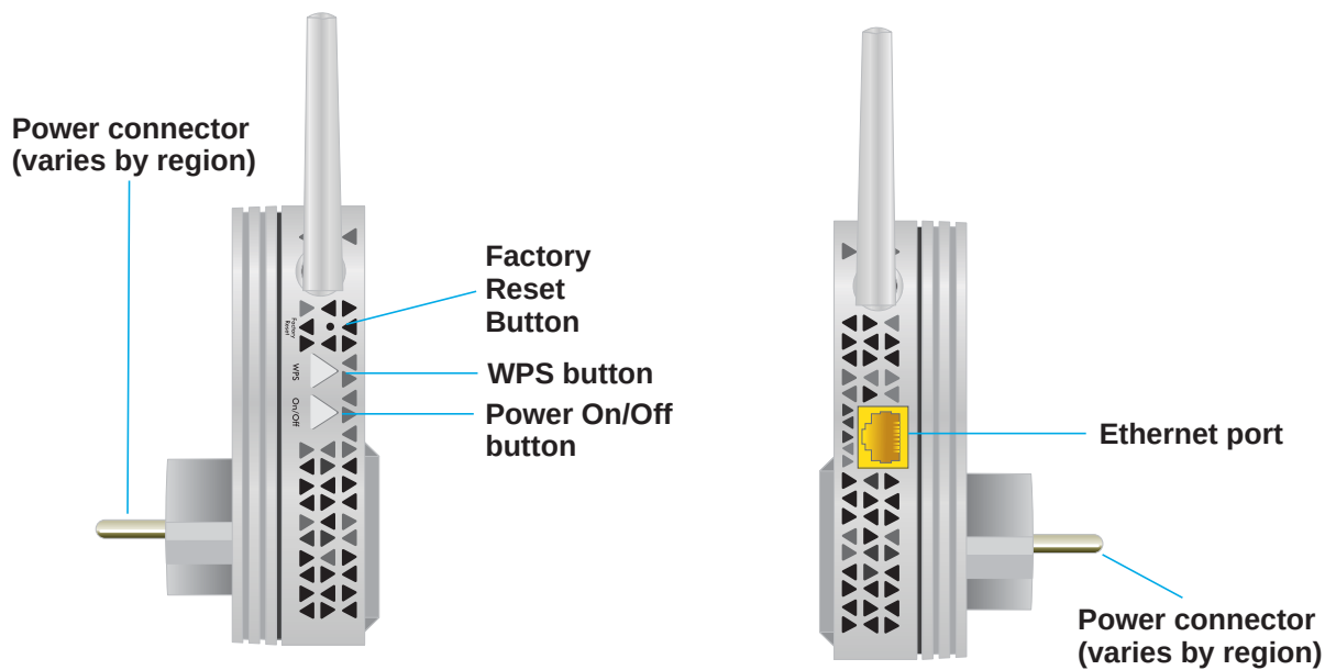
Figure 2. Side panel buttons and port
